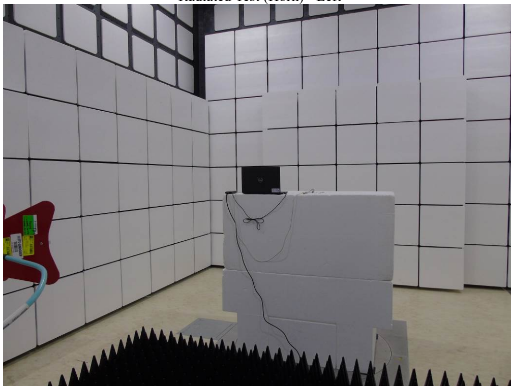
Radiated Test (Horn) - Left
