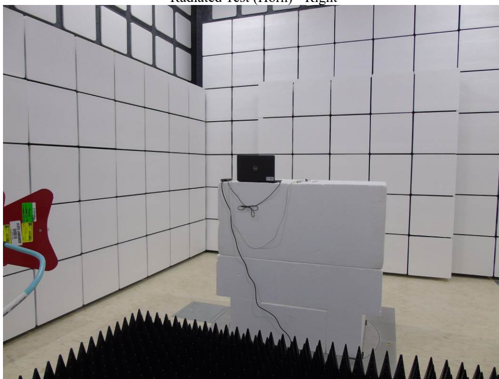
Radiated Test (Horn) - Right
