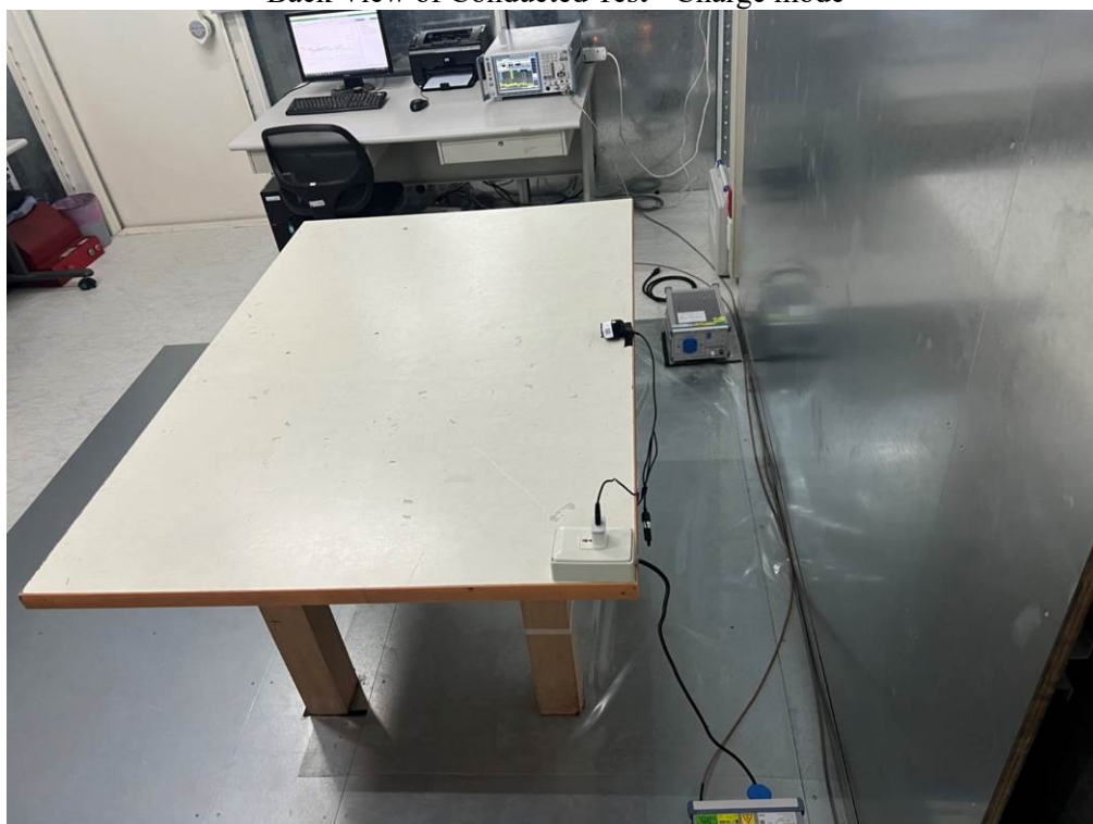
Back View of Conducted Test - Charge mode
