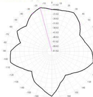
5850.0MHz Total(E2), Max=-12.89dBi
