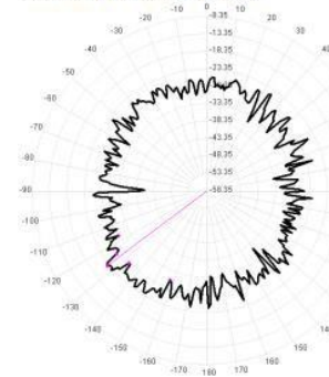
2450.0MHz Total(H), Max=-22.72dBi
