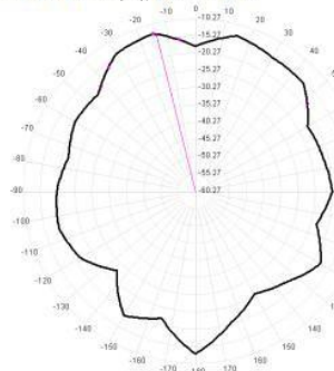
5750.0MHz Total(E2), Max=-13.01dBi
