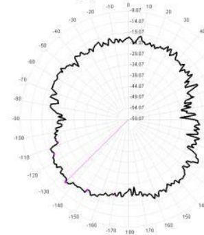
2400.0MHz Total(H), Max=-18.22dBi
