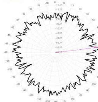
5750.0MHz Total(H), Max=-13.45dBi
