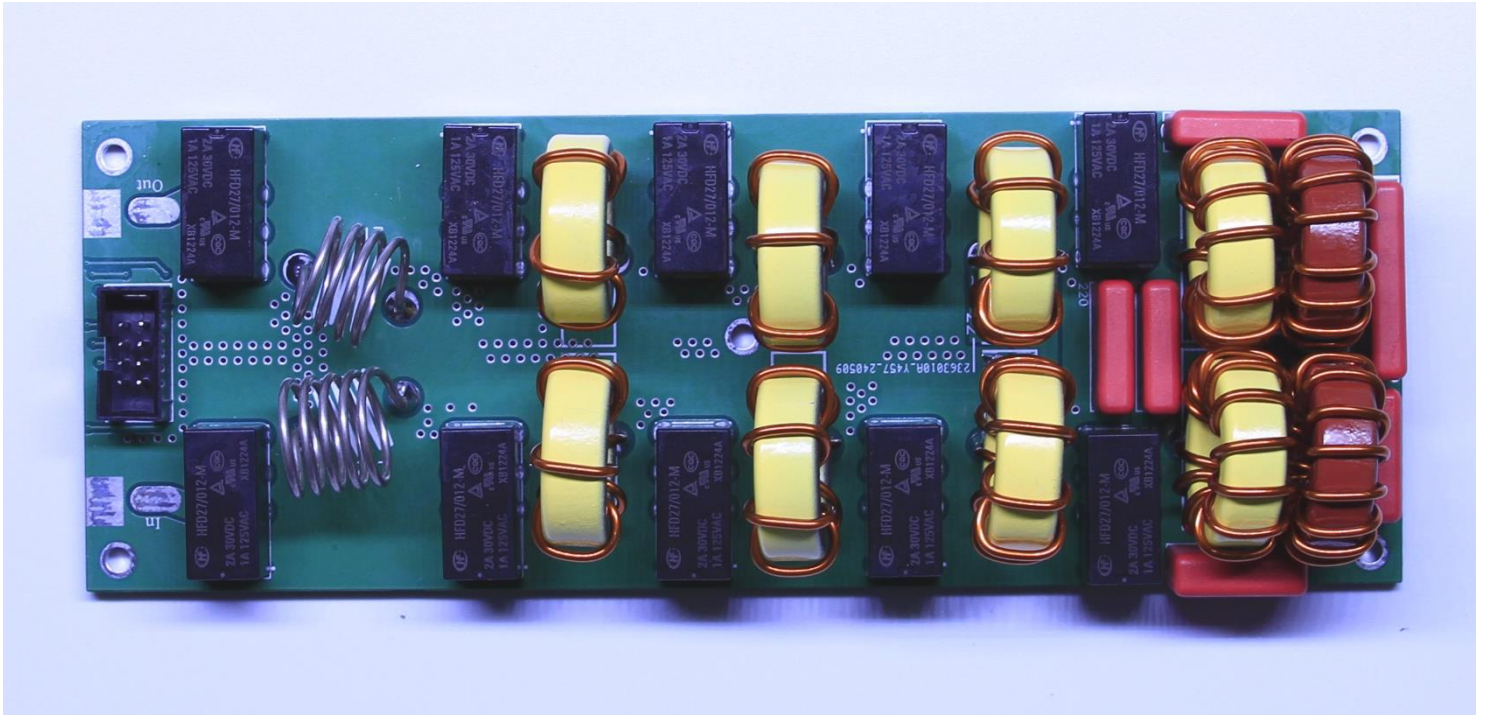
Low Pass Filter Top View
