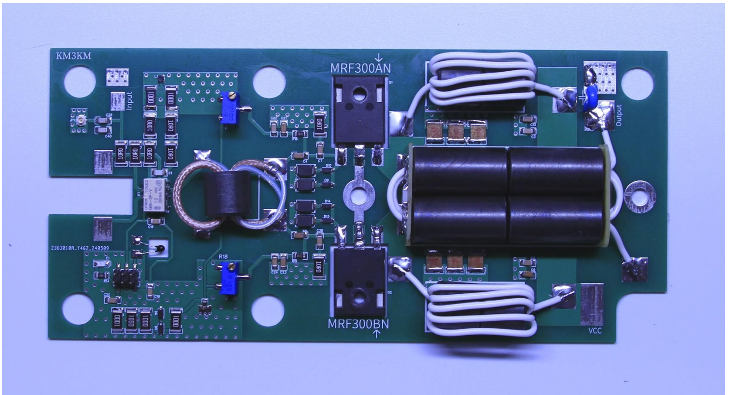
Power Unit Top View
