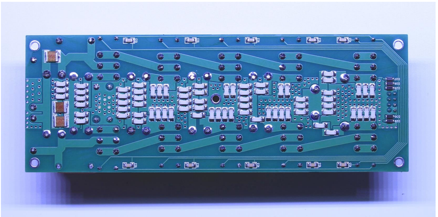
Low Pass Filter Bottom View
