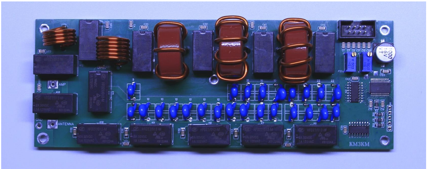
Antenna Tuner Top View
