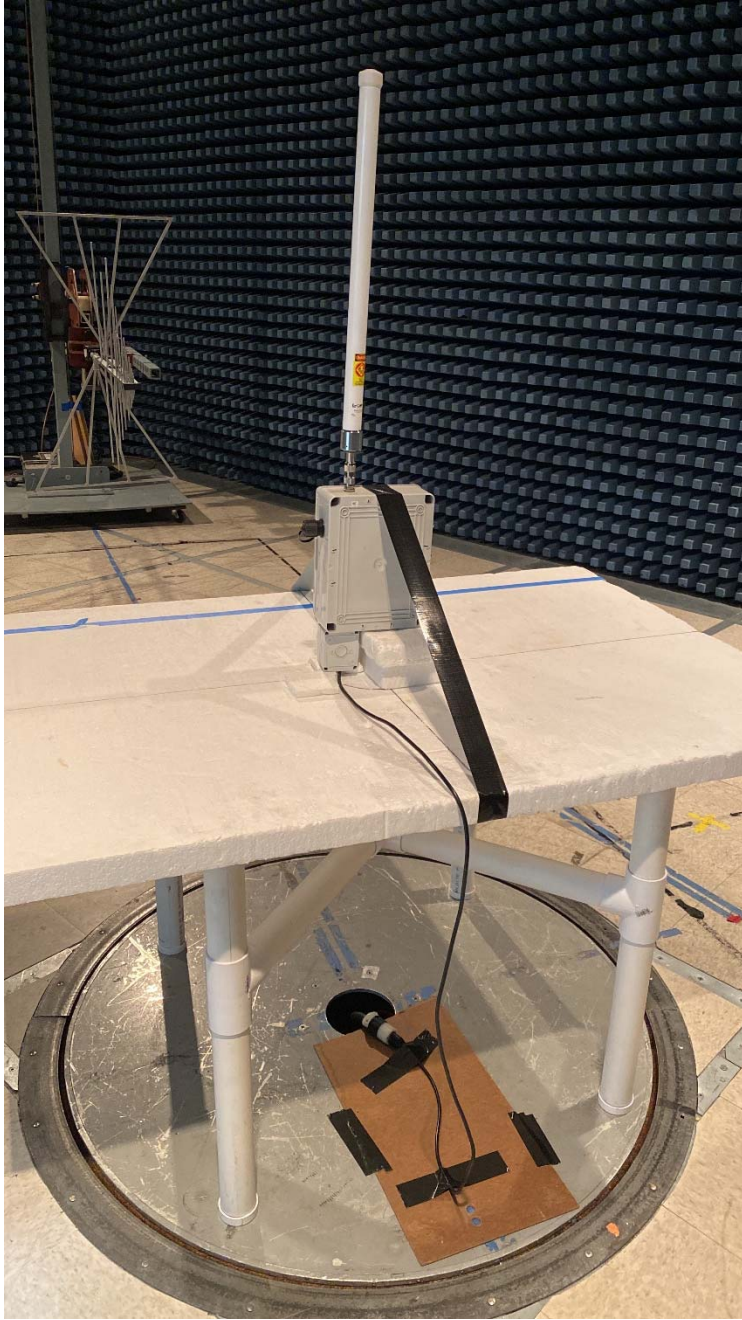
Radiated Emissions Setup, 30MHz to 1GHz (closeup)
