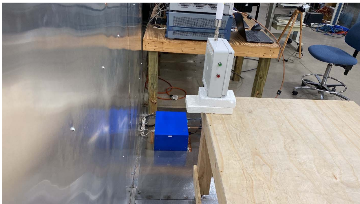
AC Line Conducted Emissions setup, back view
