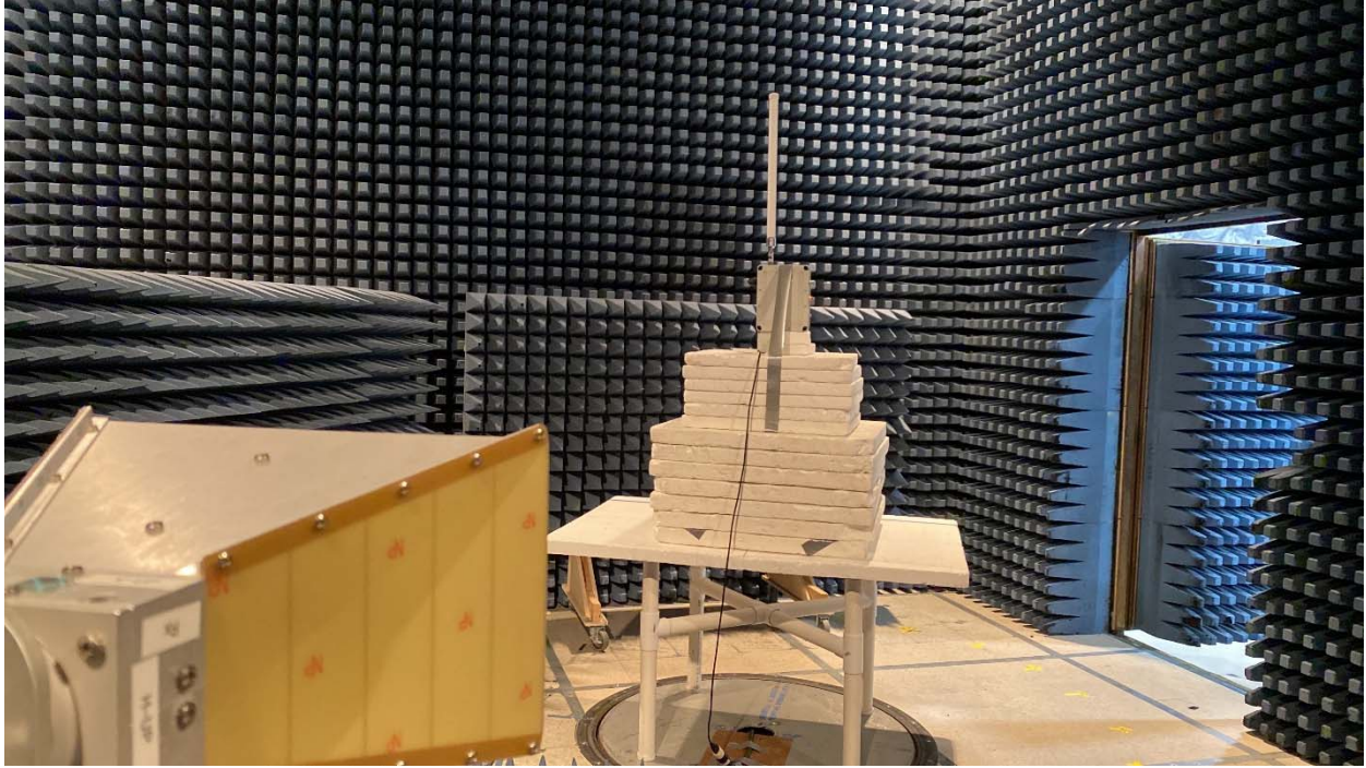
Radiated Emissions setup > 1GHz
