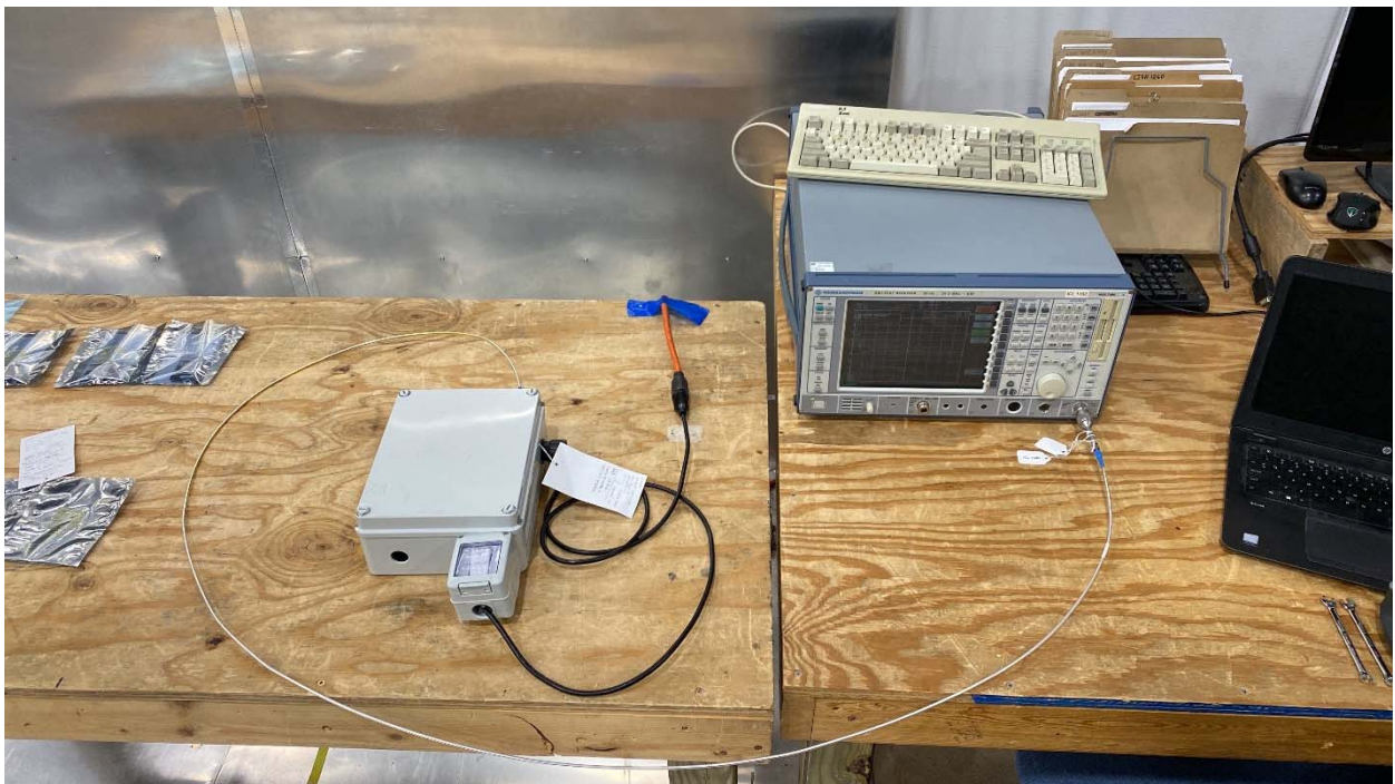
Antenna Port Conducted Emissions setup
