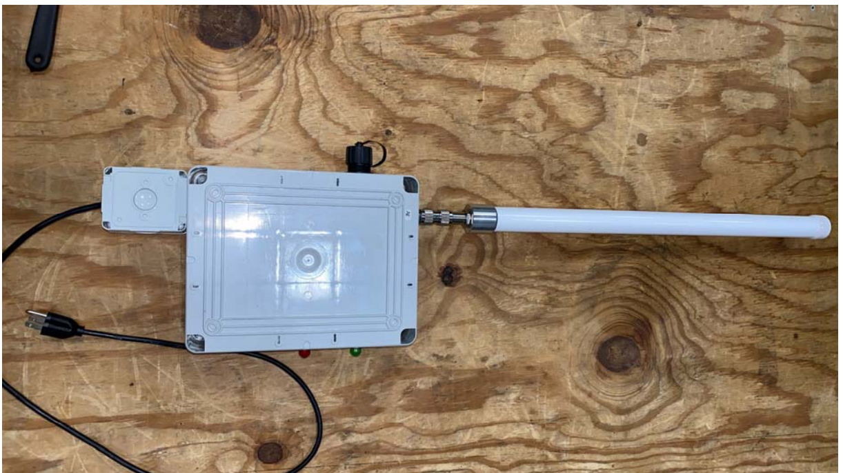
HIFIS1 Back with 6dBi Antenna
