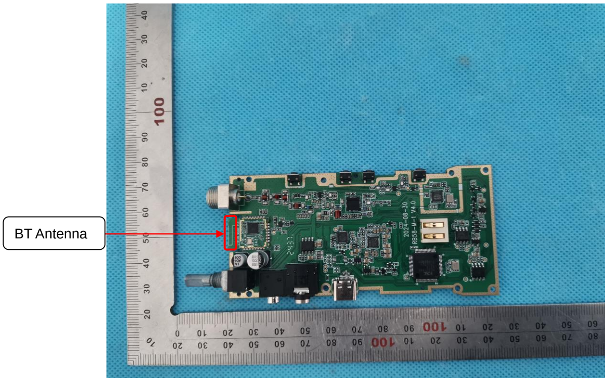
INTERNAL VIEW OF EUT (FIGURE 4)
