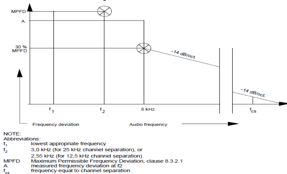
Figure 1: Frequency deviation
