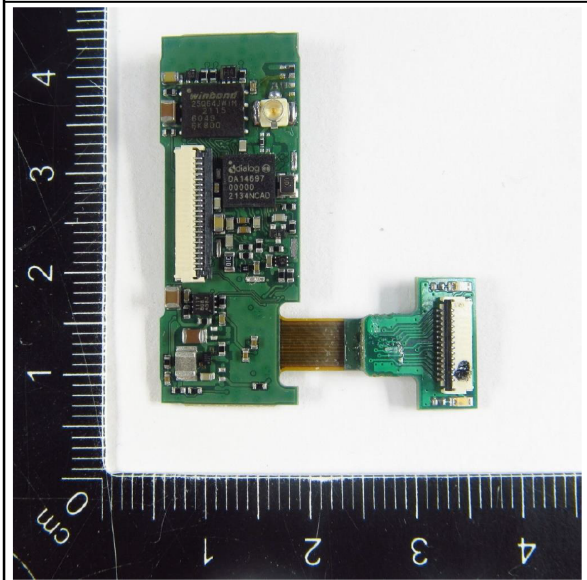
EUT top view without shield
