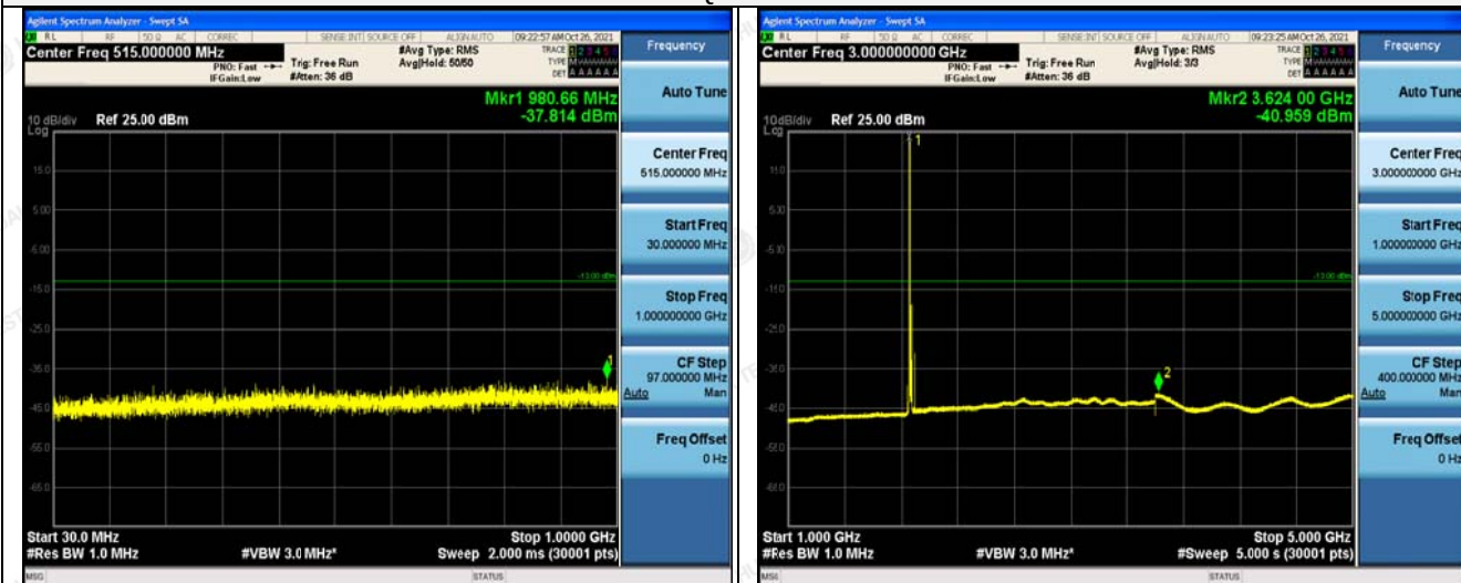
30MHz~1GHz
