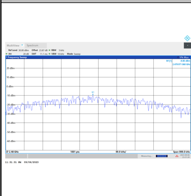
Power Density (dBm/3kHz) Plot Channel 39
