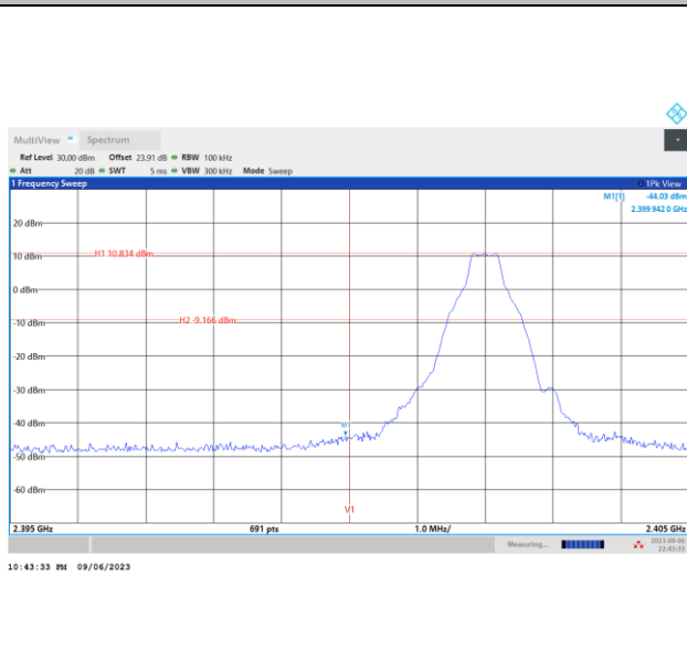
Low Band Edge Plot on Channel 00
