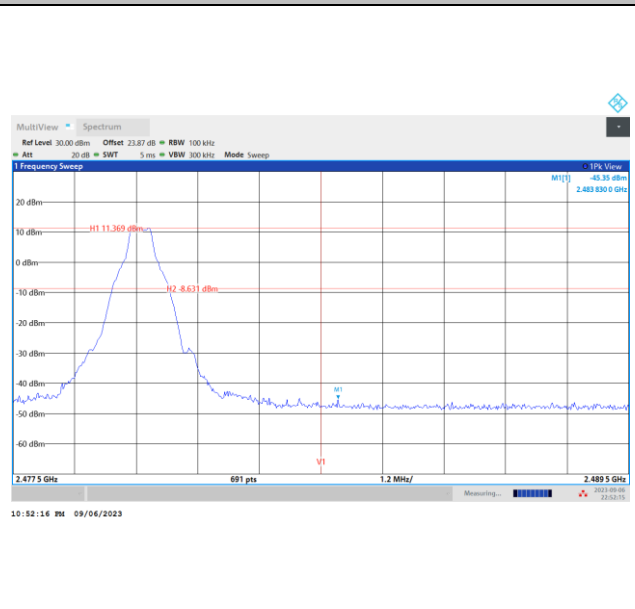
High Band Edge Plot on Channel 78
