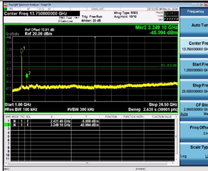
11N40SISO_Ant1_2452_0~Reference
