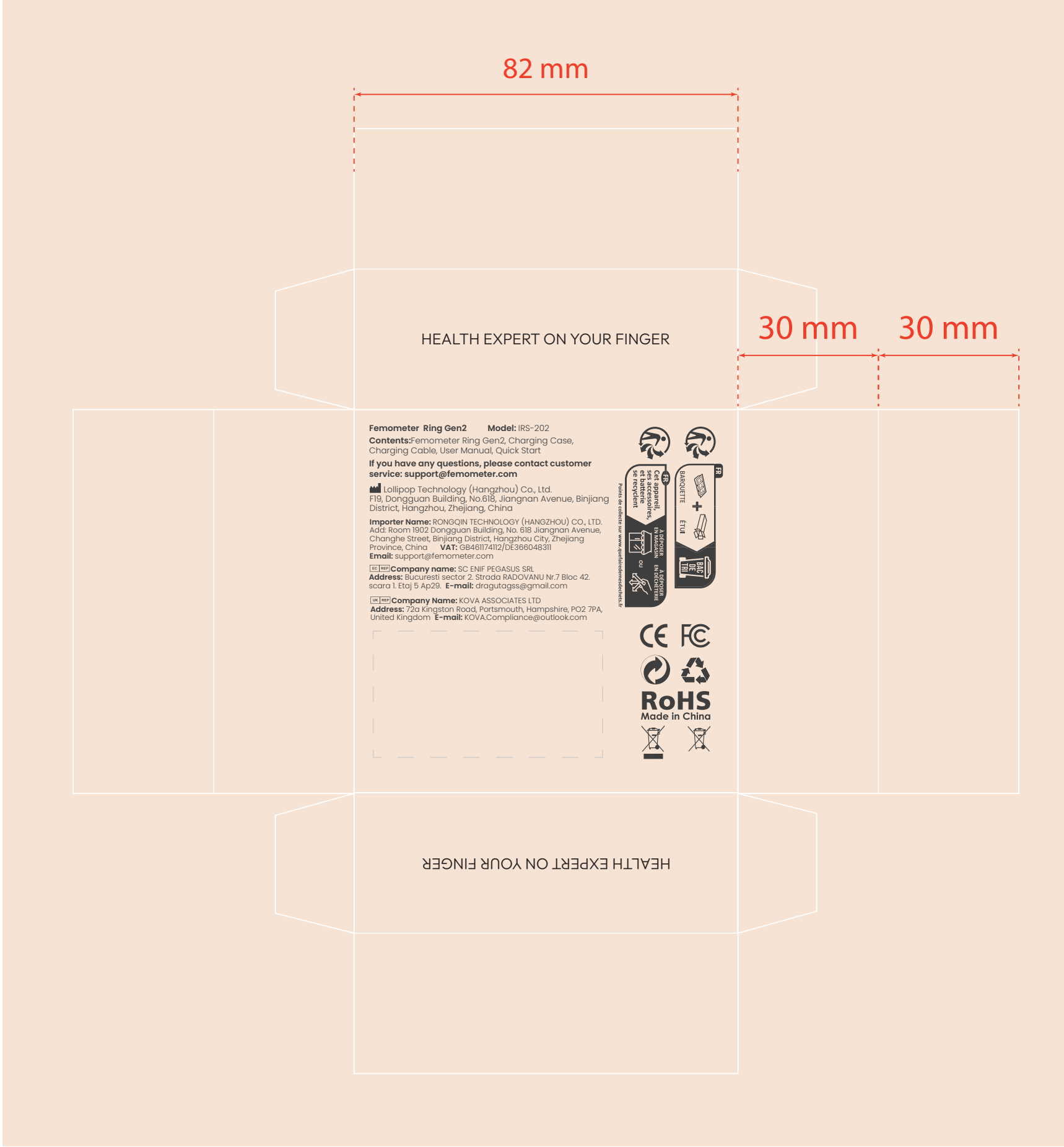
Bottom cover
