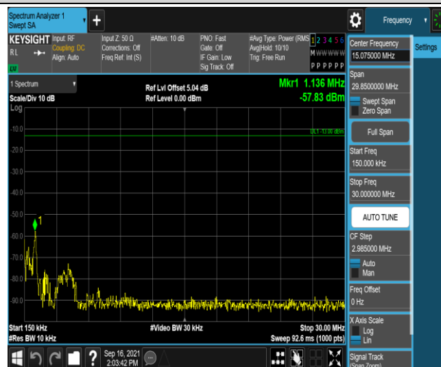
Band12-5MHz-16QAM-23095-1RB#0-Range2:0.15~30MHz
