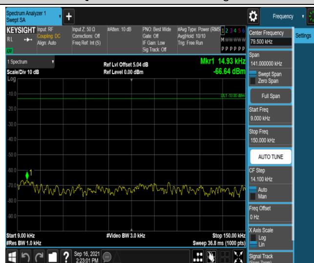
Band12-10MHz-QPSK-23060-1RB#0-Range1:0.009~0.15MHz
