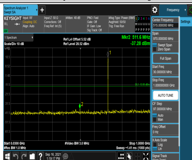
Band12-1.4MHz-16QAM-23095-1RB#0-Range3:30~1000MHz
