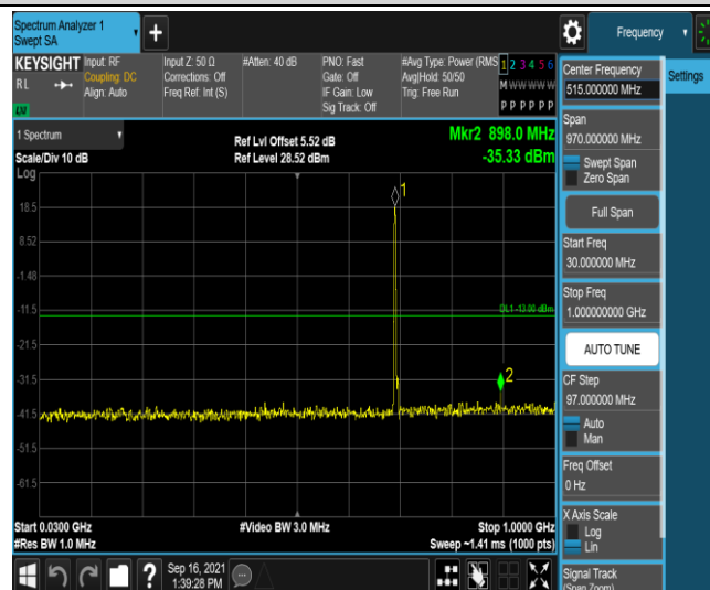
Band12-3MHz-16QAM-23025-1RB#0-Range3:30~1000MHz
