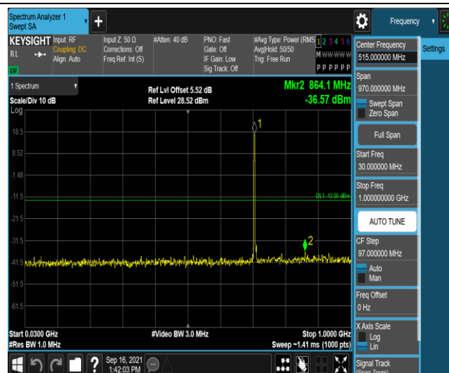
Band12-3MHz-QPSK-23165-1RB#0-Range3:30~1000MHz
