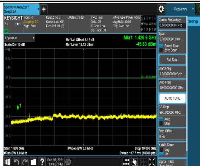
Band12-3MHz-16QAM-23165-1RB#0-Range4:1000~10000MHz
