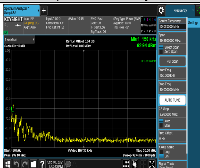
Band12-3MHz-16QAM-23165-1RB#0-Range2:0.15~30MHz
