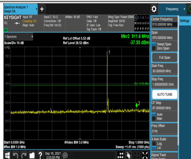
Band12-5MHz-16QAM-23095-1RB#0-Range3:30~1000MHz
