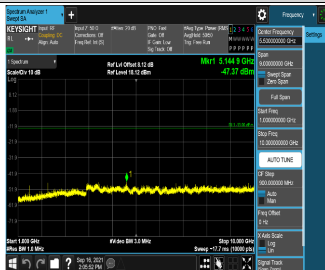
Band12-5MHz-16QAM-23155-1RB#0-Range4:1000~10000MHz
