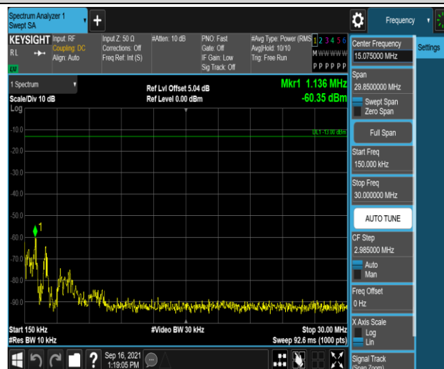
Band12-1.4MHz-16QAM-23095-1RB#0-Range2:0.15~30MHz
