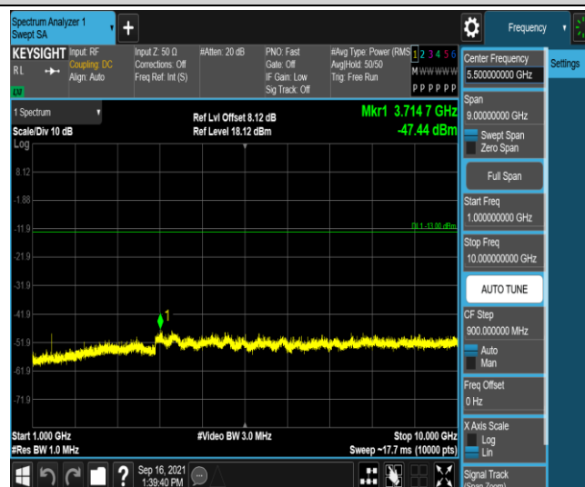
Band12-3MHz-16QAM-23025-1RB#0-Range4:1000~10000MHz
