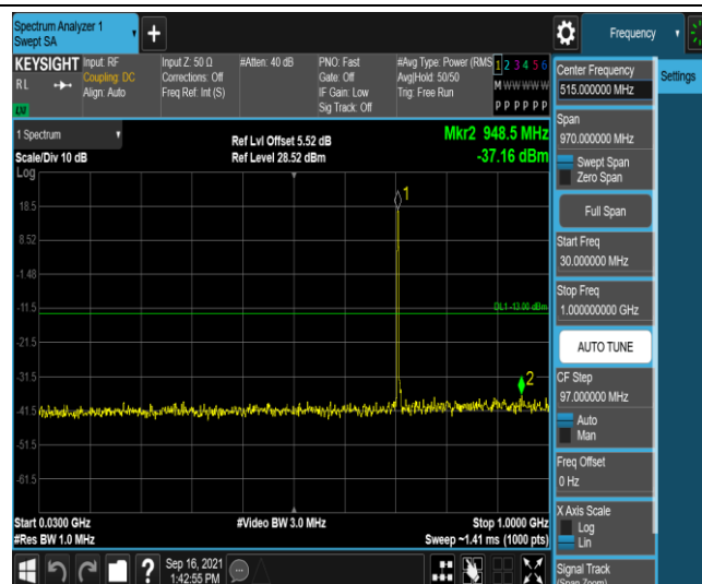
Band12-3MHz-16QAM-23165-1RB#0-Range3:30~1000MHz
