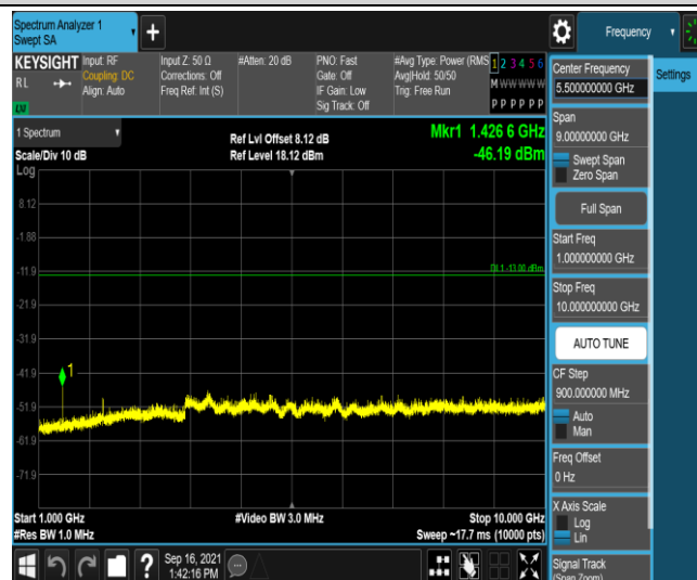
Band12-3MHz-QPSK-23165-1RB#0-Range4:1000~10000MHz
