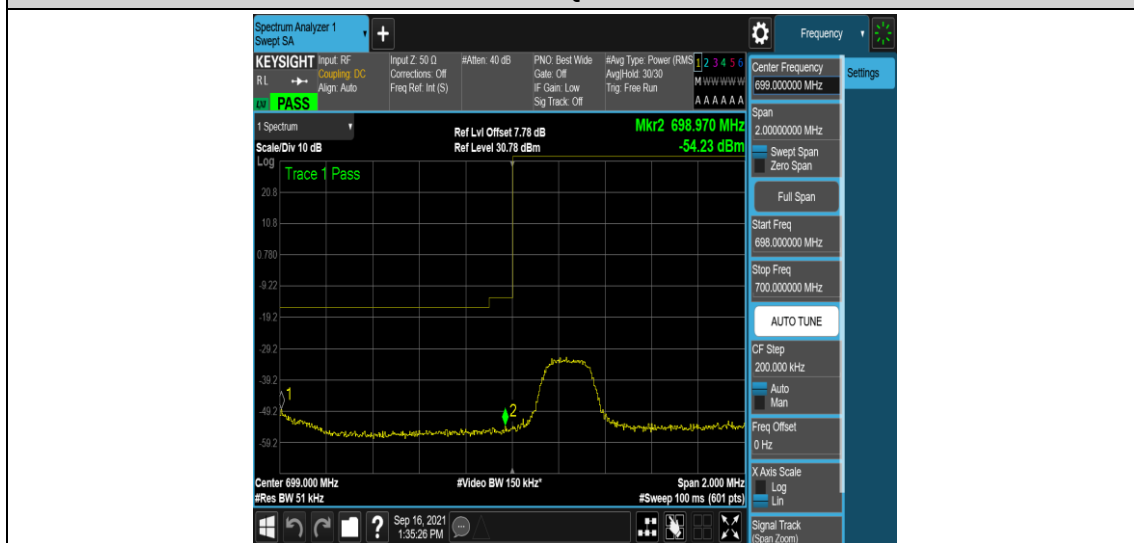
Band12-3MHz-16QAM-23025-1RB#14
