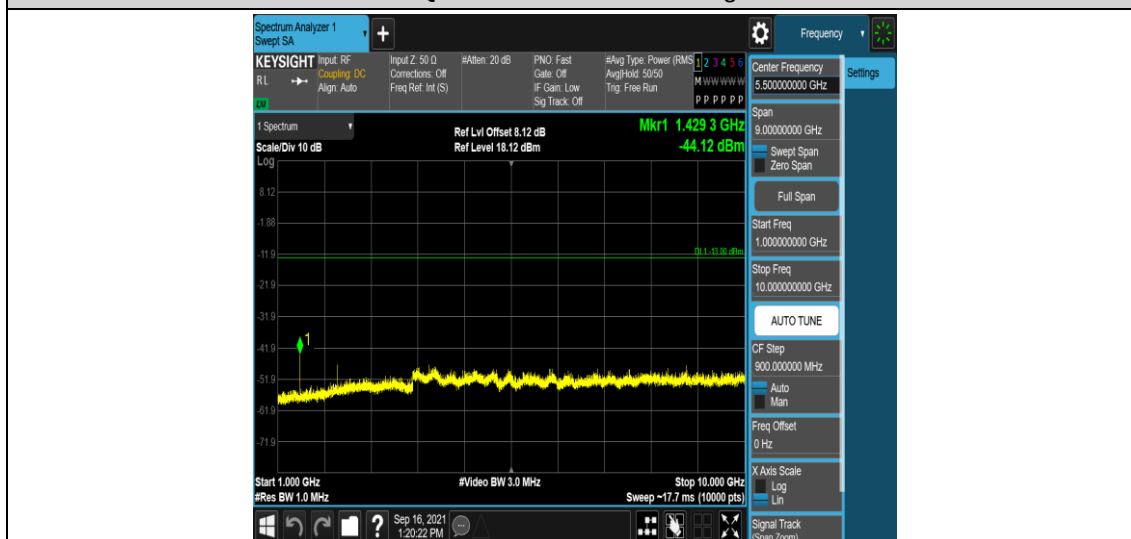
Band12-1.4MHz-QPSK-23173-1RB#0-Range4:1000~10000MHz
