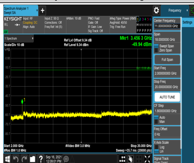
Band4-10MHz-16QAM-20175-1RB#0-Range5:2000~20000MHz
