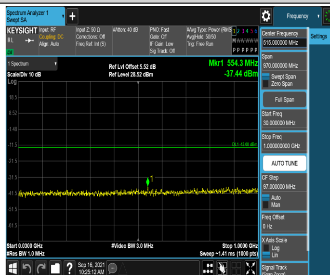
Band4-1.4MHz-16QAM-20393-1RB#0-Range3:30~1000MHz
