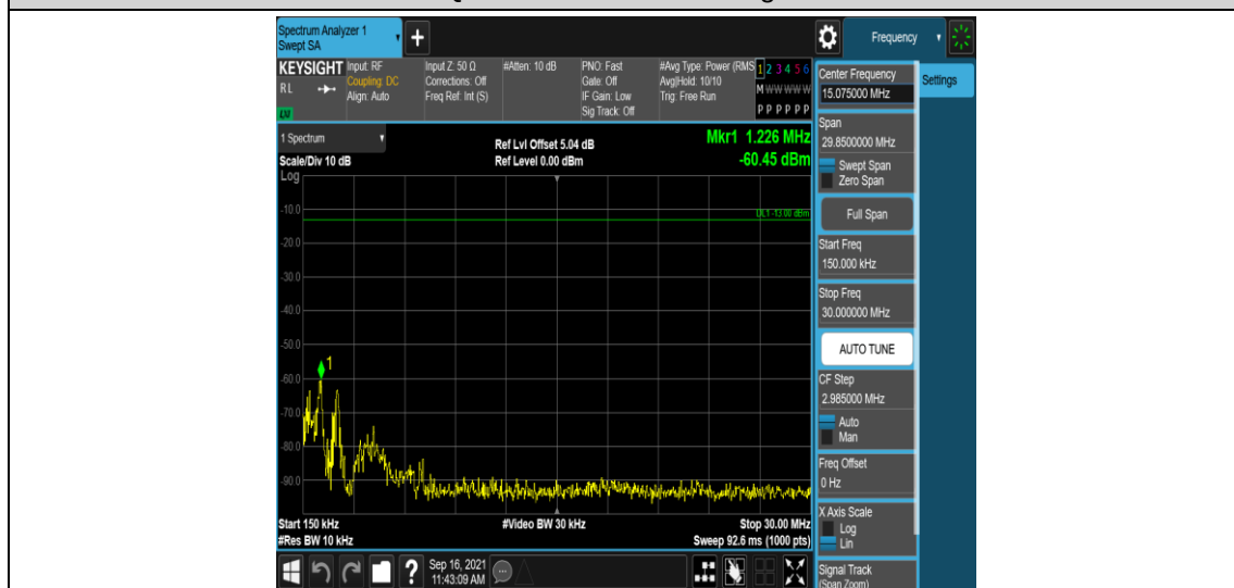
Band4-5MHz-16QAM-20175-1RB#0-Range2:0.15~30MHz
