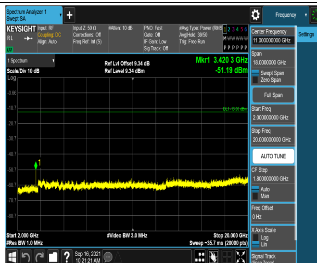
Band4-1.4MHz-16QAM-19957-1RB#0-Range5:2000~20000MHz
