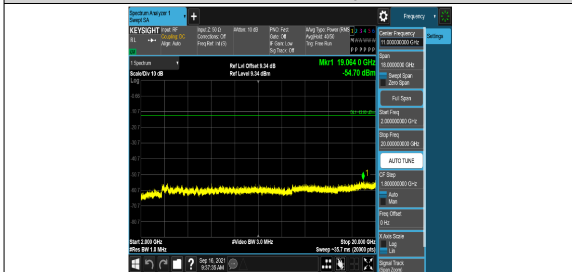
Band2-15MHz-QPSK-19125-1RB#0-Range5:2000~20000MHz
