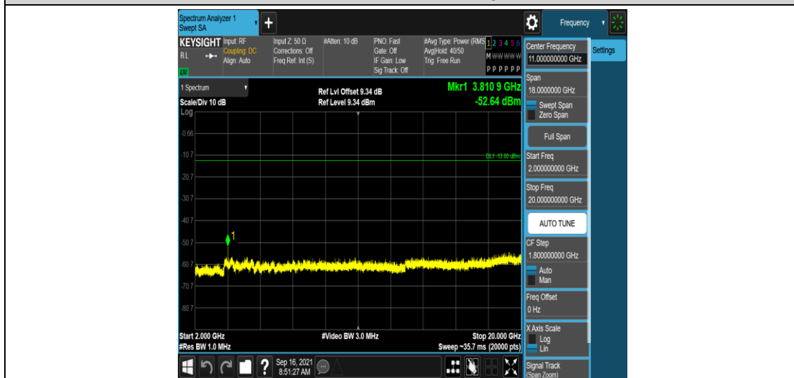
Band2-5MHz-16QAM-19175-1RB#0-Range5:2000~20000MHz
