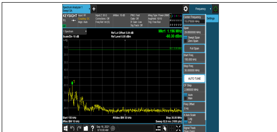
Band2-10MHz-16QAM-18650-1RB#0-Range2:0.15~30MHz
