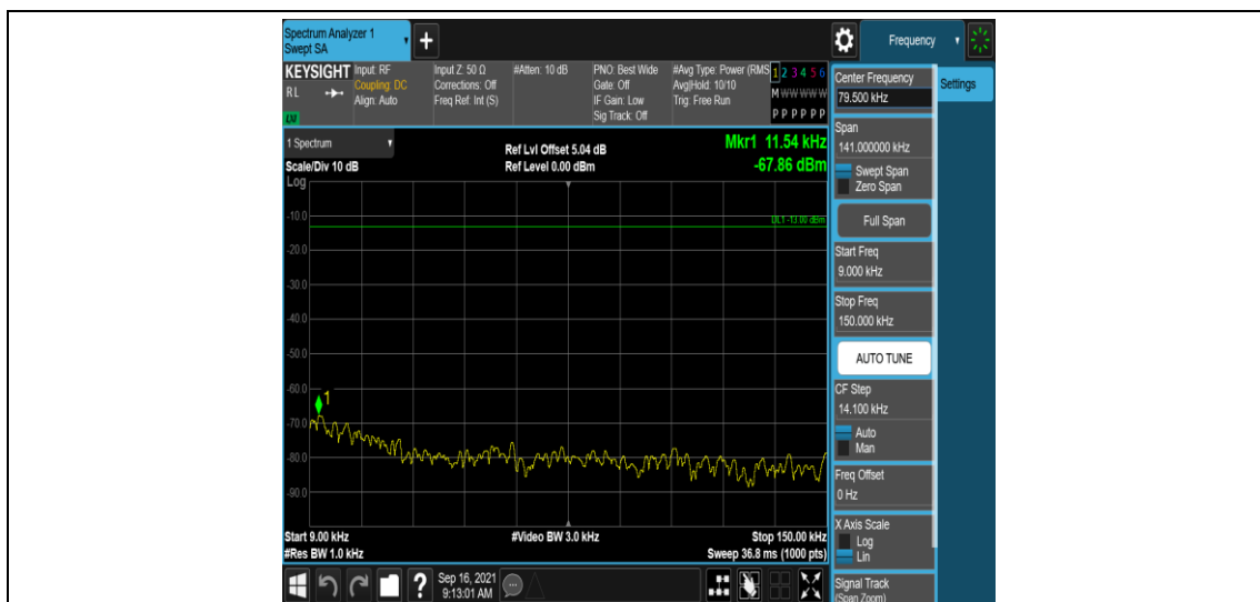
Band2-10MHz-QPSK-19150-1RB#0-Range1:0.009~0.15MHz
