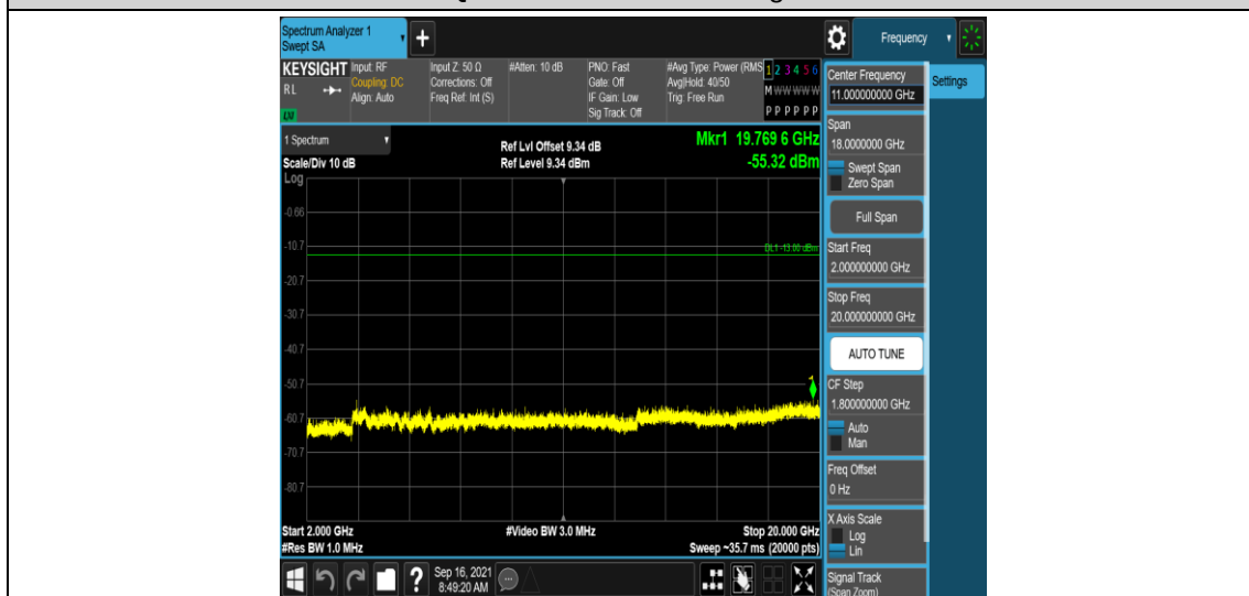
Band2-5MHz-16QAM-18900-1RB#0-Range5:2000~20000MHz
