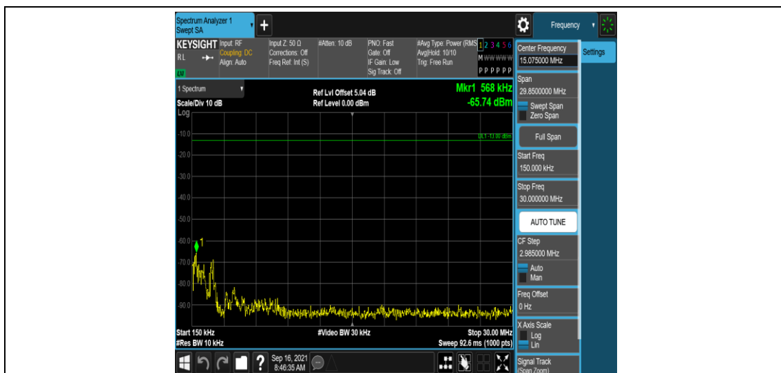
Band2-5MHz-16QAM-18625-1RB#0-Range2:0.15~30MHz
