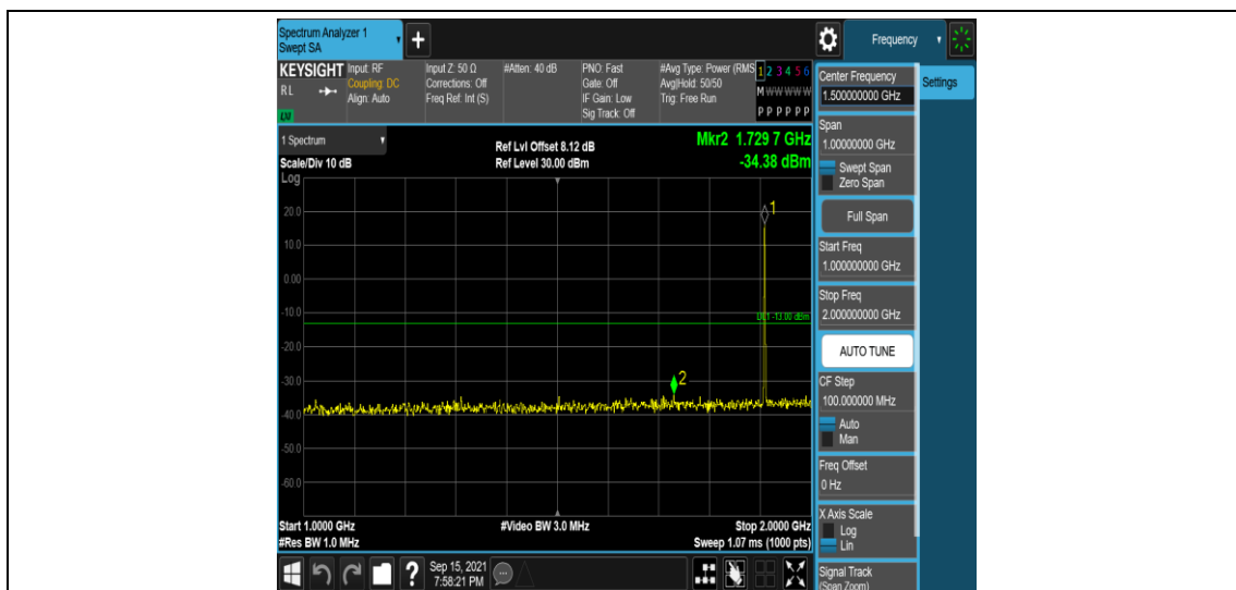
Band2-1.4MHz-16QAM-19193-1RB#0-Range4:1000~2000MHz
