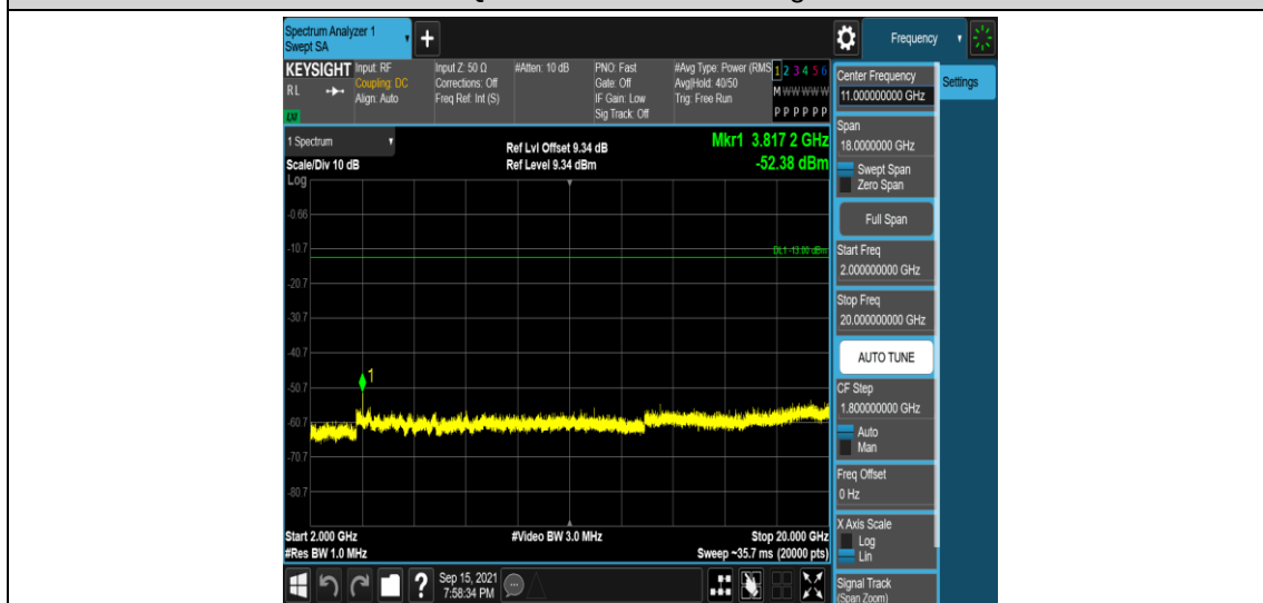
Band2-1.4MHz-16QAM-19193-1RB#0-Range5:2000~20000MHz
