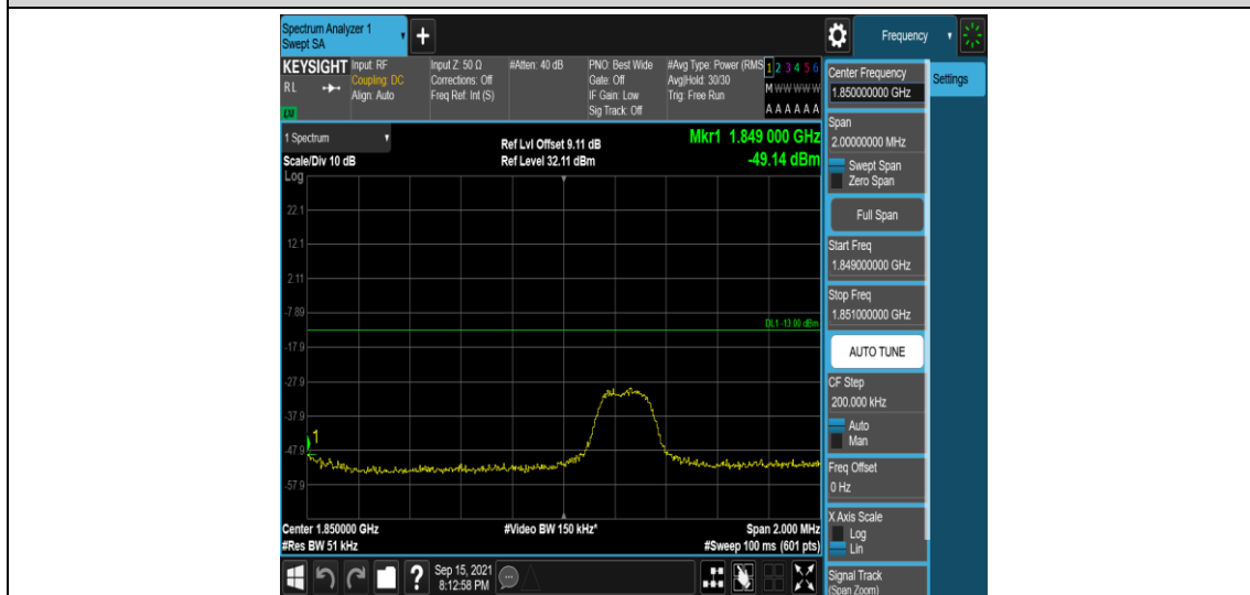
Band2-3MHz-16QAM-18615-1RB#14
