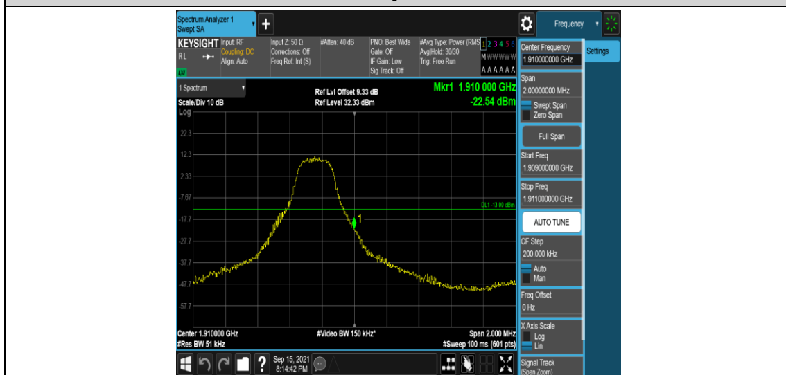
Band2-3MHz-16QAM-19185-1RB#14
