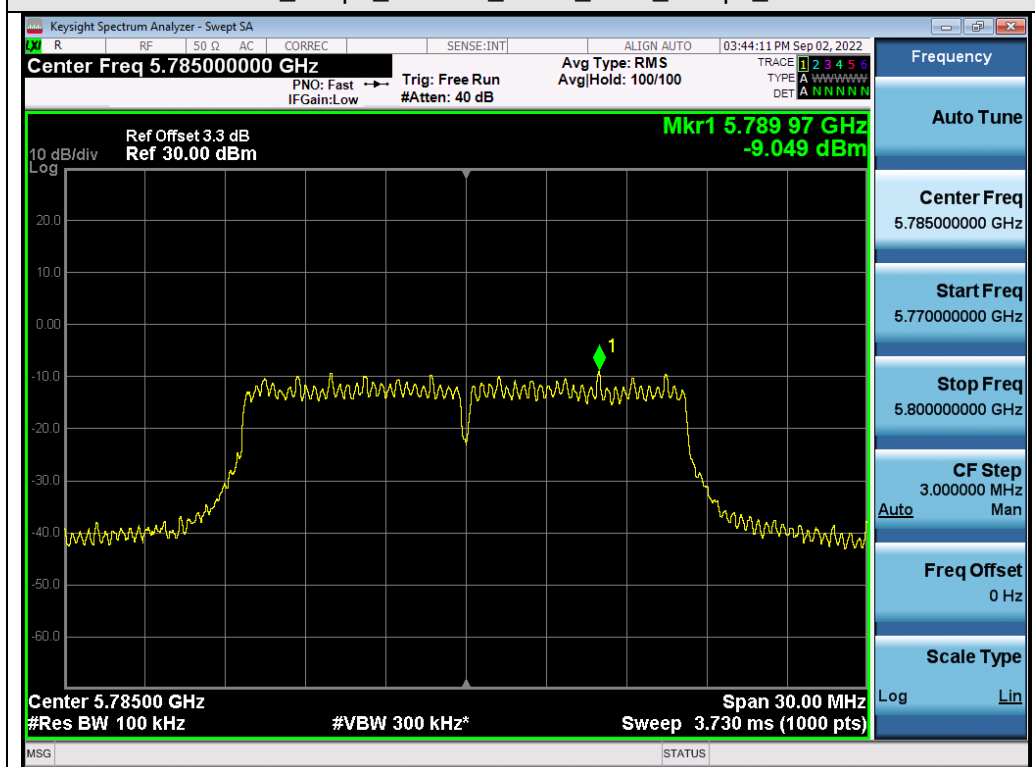
Test_Graph_802.11a_ANT1_5785_6Mbps_PSD
