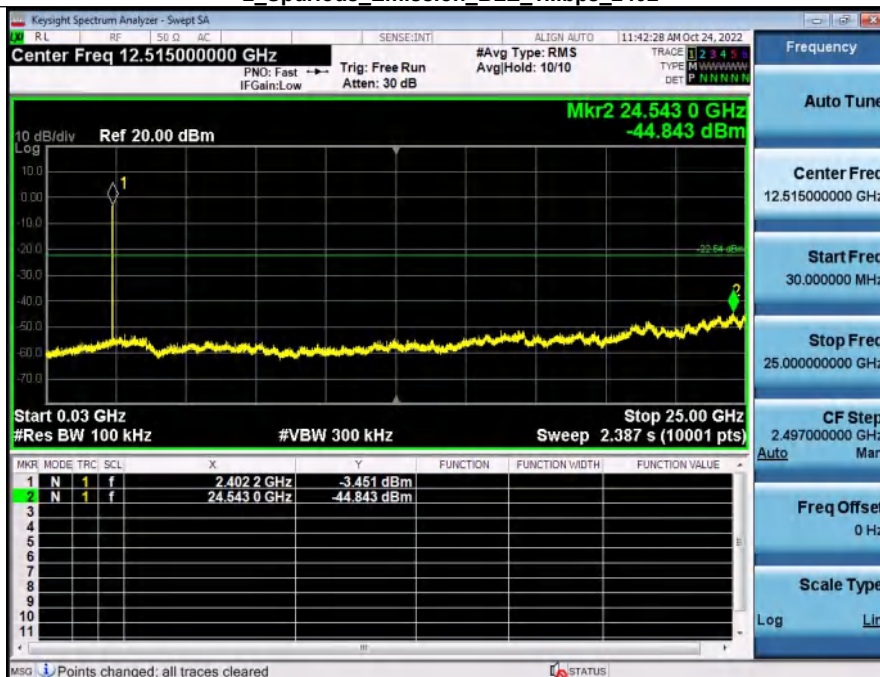
2_Spurious_Emission_BLE_1Mbps_2402
