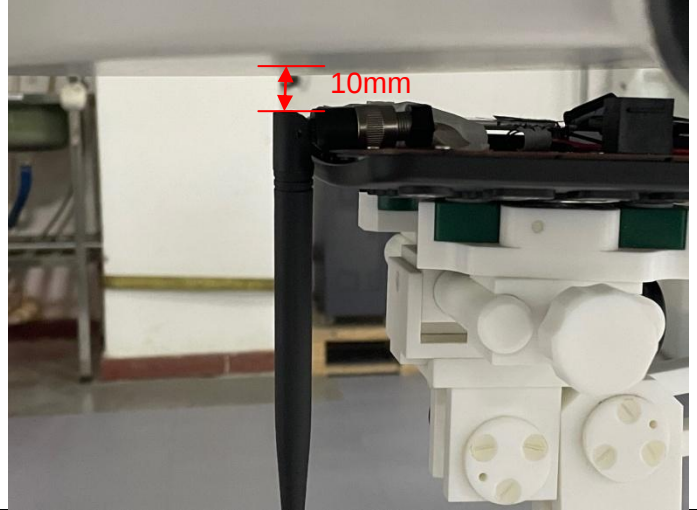
Back Side and Ant Vertical (Separation distance of 10mm)
