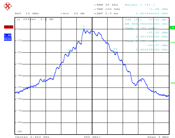
Test plots GFSK Low Channel
