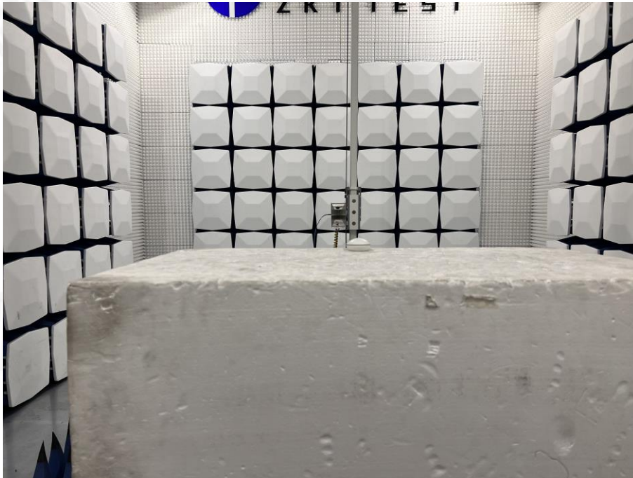
Radiated band emission (Above 1GHz):
