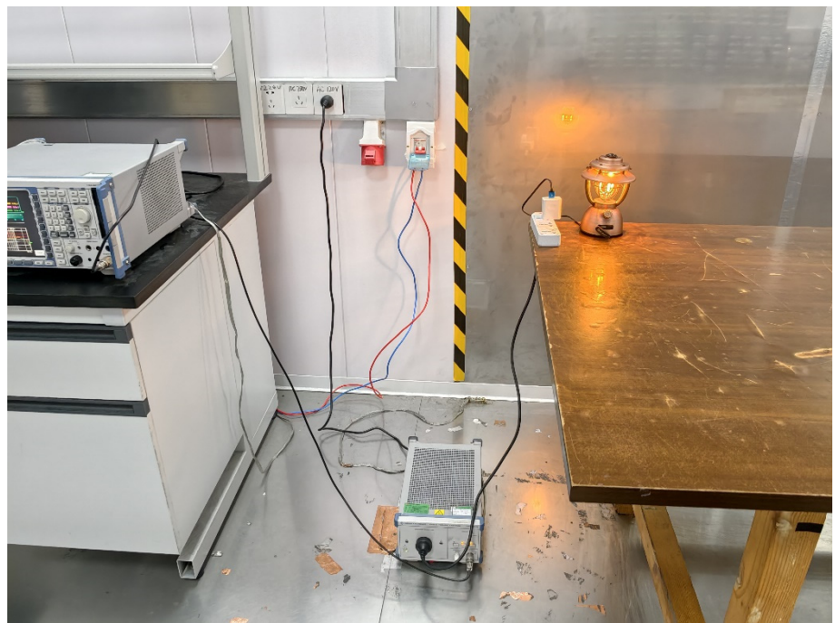
Conducted Emission Test Setup-TM3
