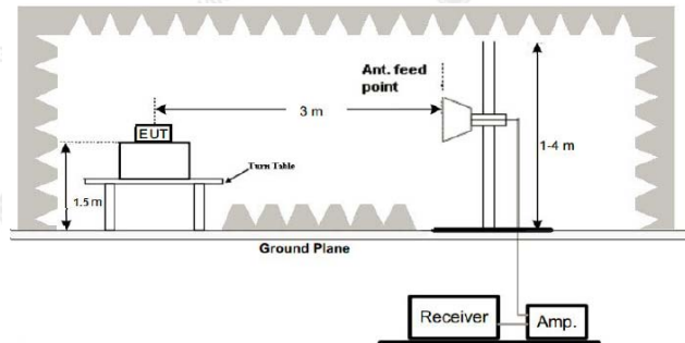
Above 1GHz
