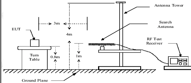
Above 1GHz
