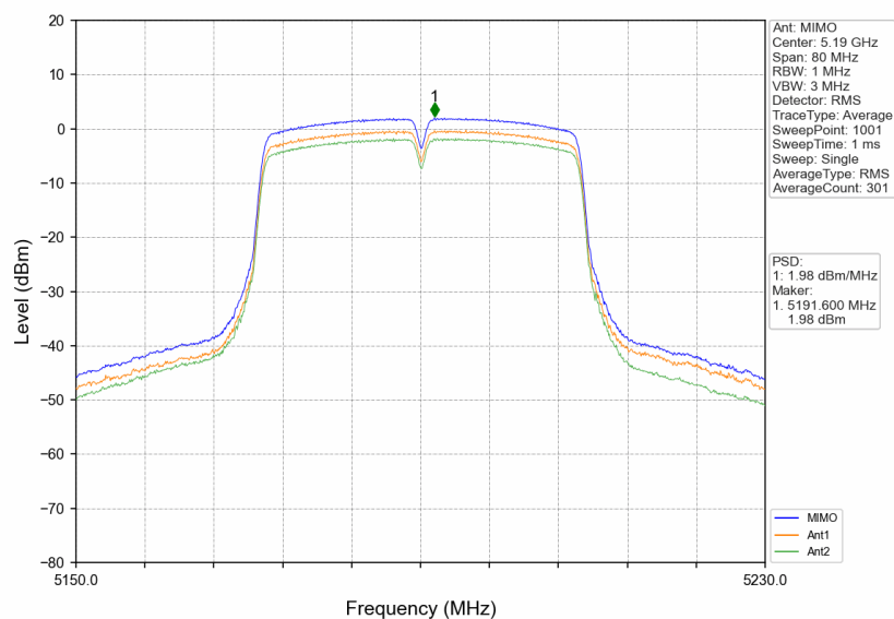
802.11n(HT40)_LCH_5190MHz_MIMO_NTNV
