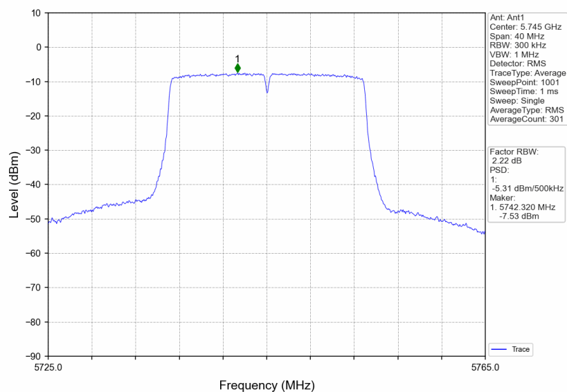
802.11ac(VHT20)_LCH_5745MHz_Ant1_NTNV
