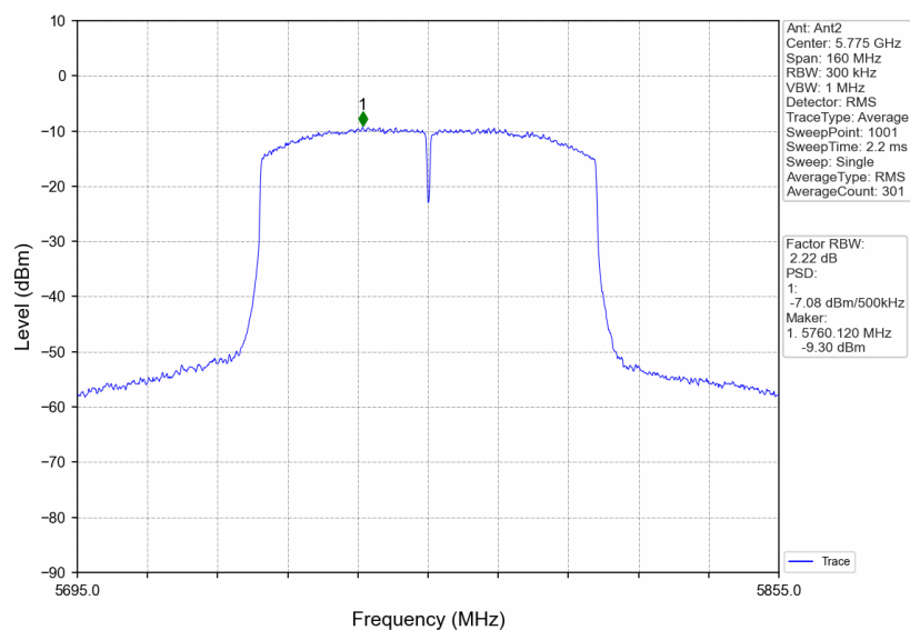
802.11ac(VHT80)_MCH_5775MHz_Ant2_NTNV
