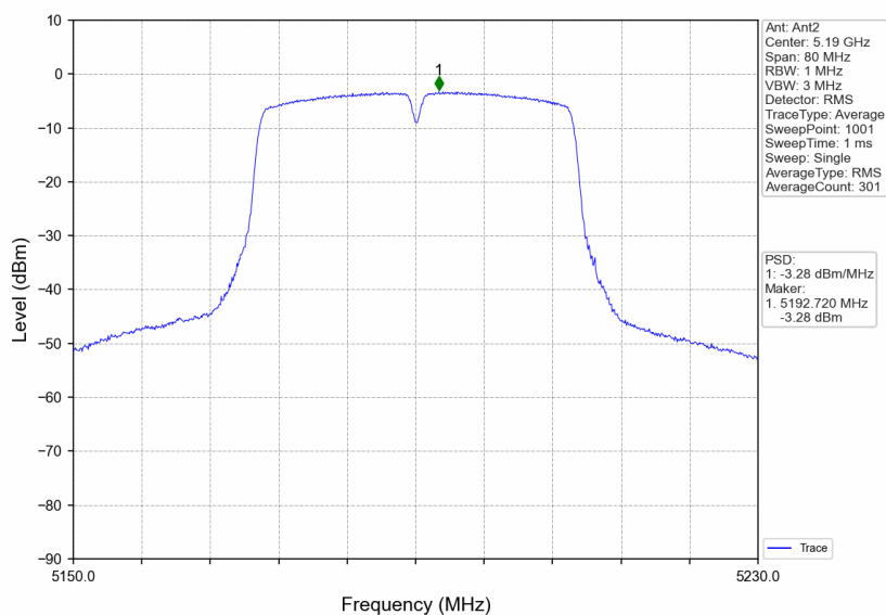
802.11ac(VHT40)_LCH_5190MHz_Ant2_NTNV
