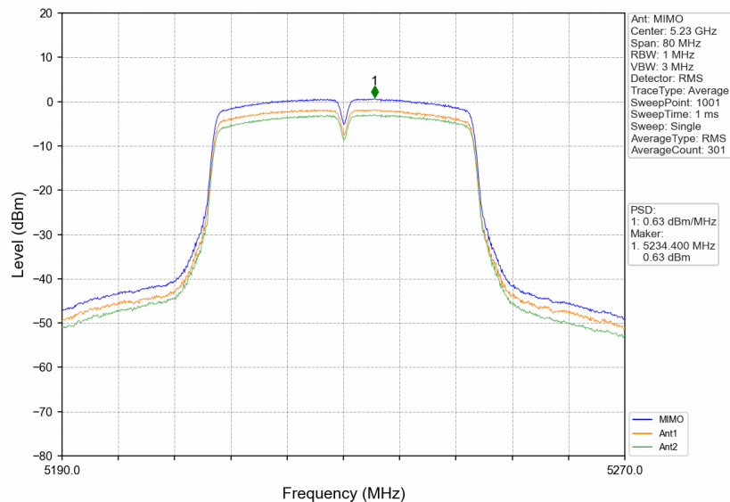
802.11ac(VHT40)_HCH_5230MHz_MIMO_NTNV
