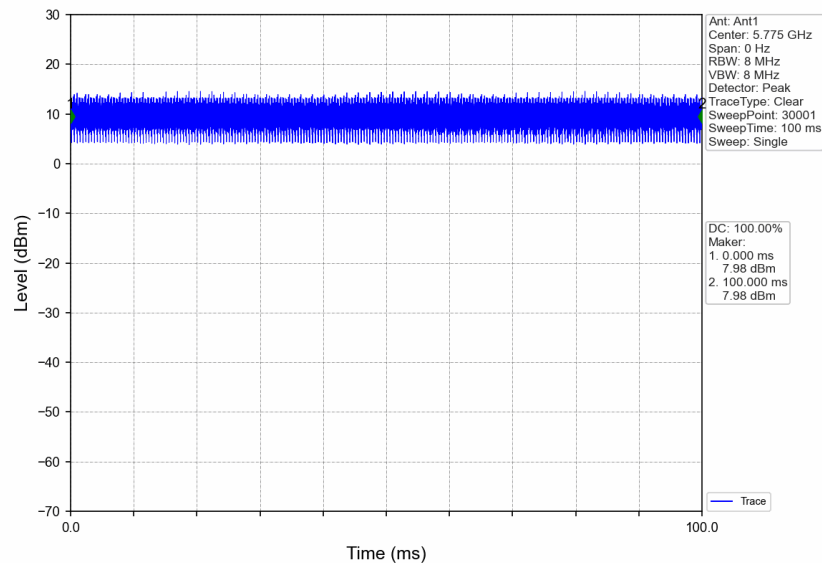
802.11ac(VHT80)_MCH_5775MHz_Ant1_NTNV
