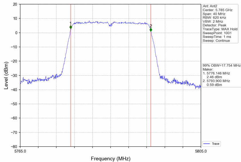
802.11n(HT20)_MCH_5785MHz_Ant2_NTNV
