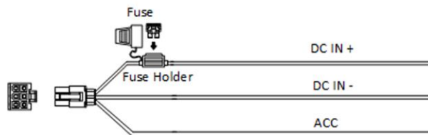
Figure 2-3 Power Cord
