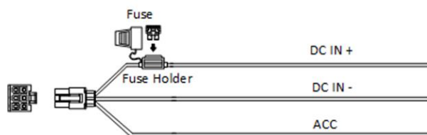
Figure 2-1 Power Cord
