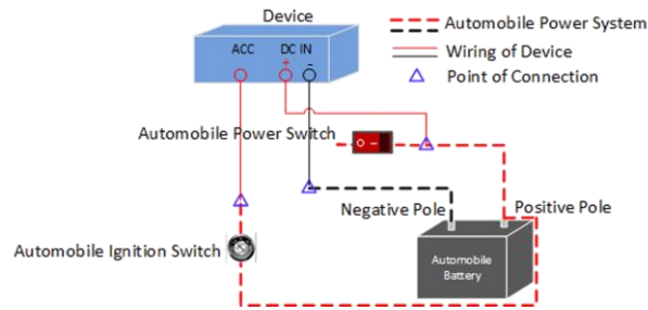
Figure 2-2 Shutdown Delay
