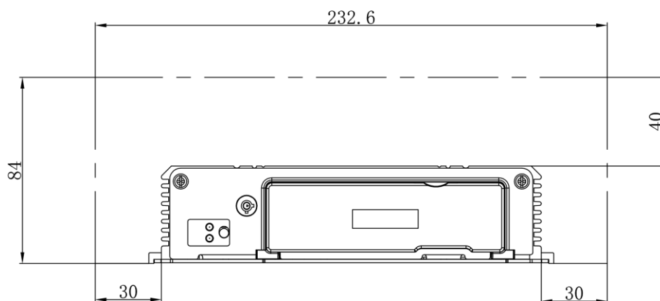
Figure 1-1 Recommended Installation Space
