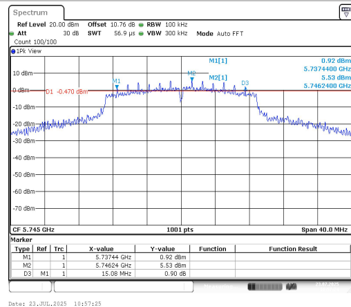
11N20SISO-Ant1-5745-PASS
