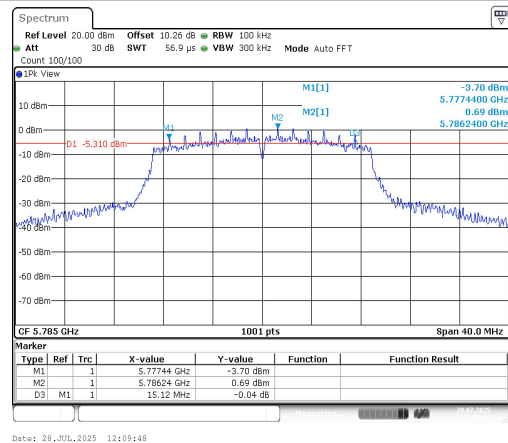
11AC20SISO-Ant1-5785-PASS
