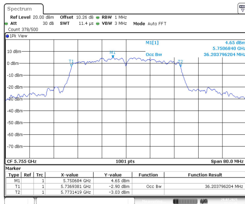
11AC40SISO-Ant1-5755
