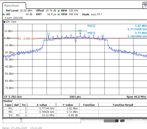
11N20SISO-Ant1-5785-PASS
