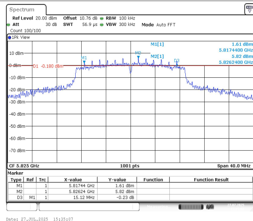
11N20SISO-Ant1-5825-PASS
