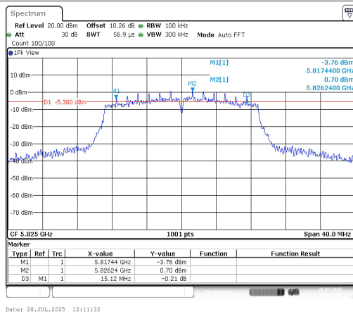
11AC20SISO-Ant1-5825-PASS
