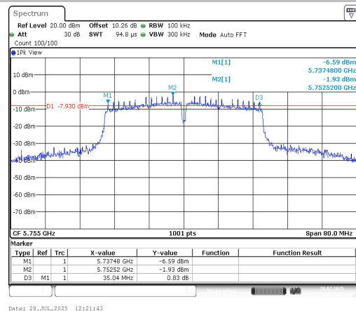
11AC40SISO-Ant1-5755-PASS
