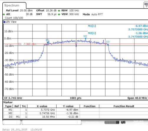
11AC20SISO-Ant1-5745-PASS
