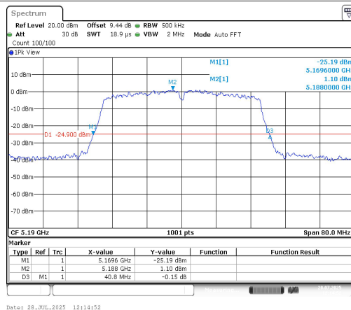
11AC40SISO-Ant1-5190
