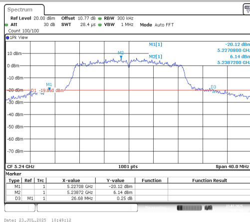
11N20SISO-Ant1-5240
