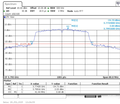
11AC40SISO-Ant1-5795
