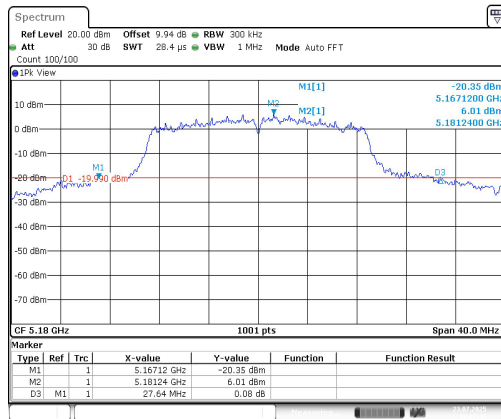
11N20SISO-Ant1-5180
