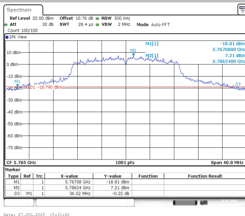
11N20SISO-Ant1-5785
