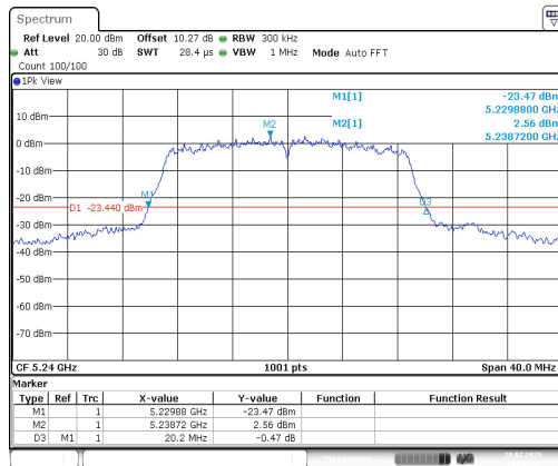
11AC20SISO-Ant1-5240
