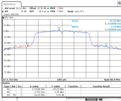
11AC40SISO-Ant1-5755
