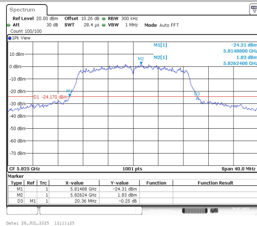
11AC20SISO-Ant1-5825
