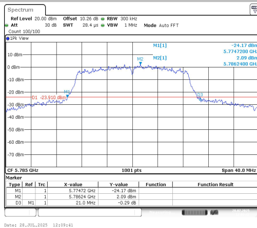
11AC20SISO-Ant1-5785
