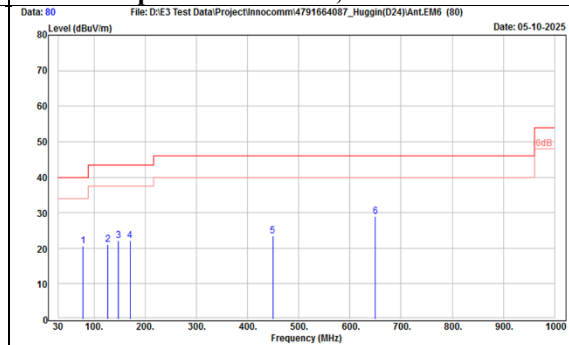
TX, Ant Plus (Ch 39) Radiated Spurious Emission, Vertical
