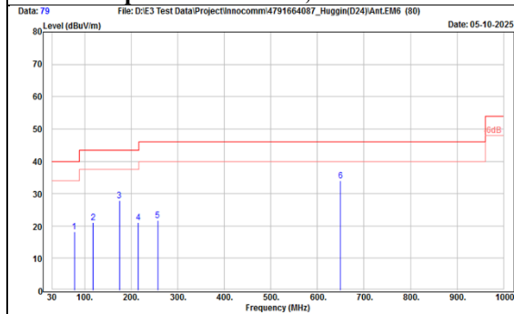
TX, Ant Plus (Ch 39) Radiated Spurious Emission, Horizontal
