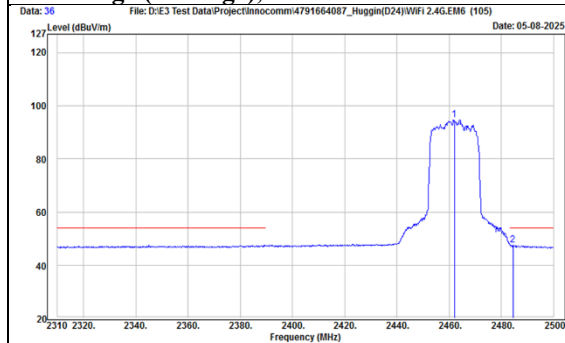
TX, 802.11ac(VHT20) (Ch 11) Band Edge (Peak), Horizontal
