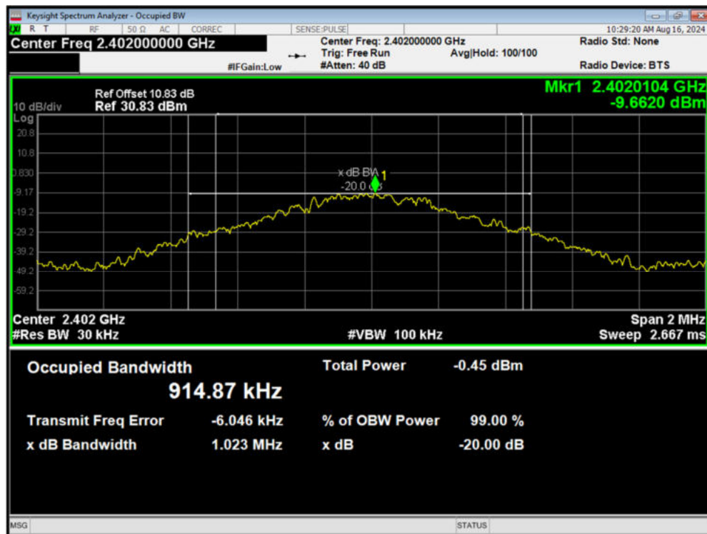
-20dB Bandwidth 1-DH5 2402MHz
