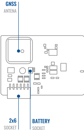
TOP VIEW (WITHOUT COVER)
