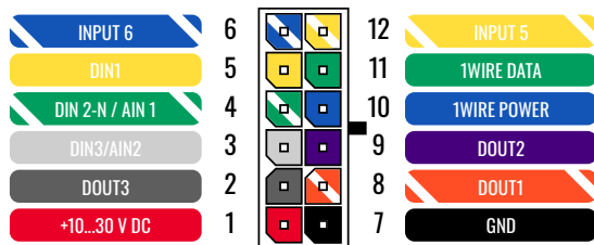
FMC13A 2x6 socket pinout
