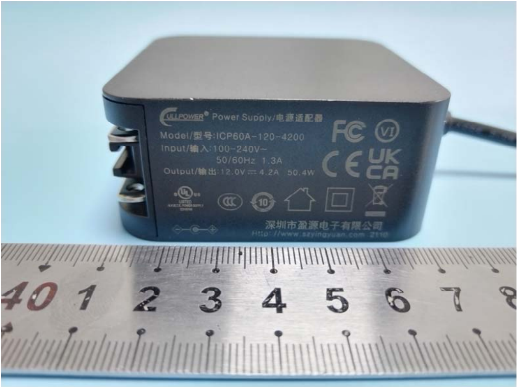
Adapter 2
