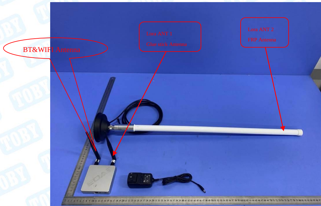
Photo 1 Appearance of EUT
