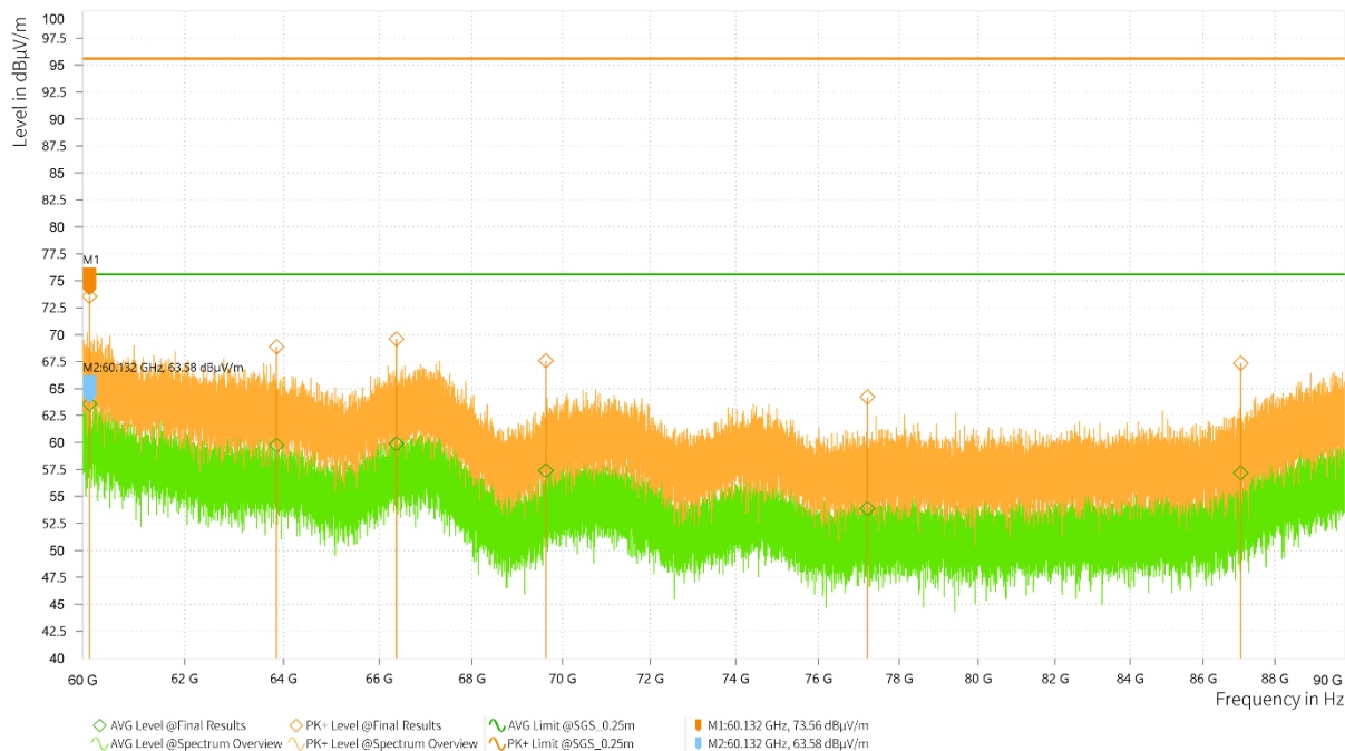
Antenna Polarity & Test Distance: Vertical at 0.25 m
