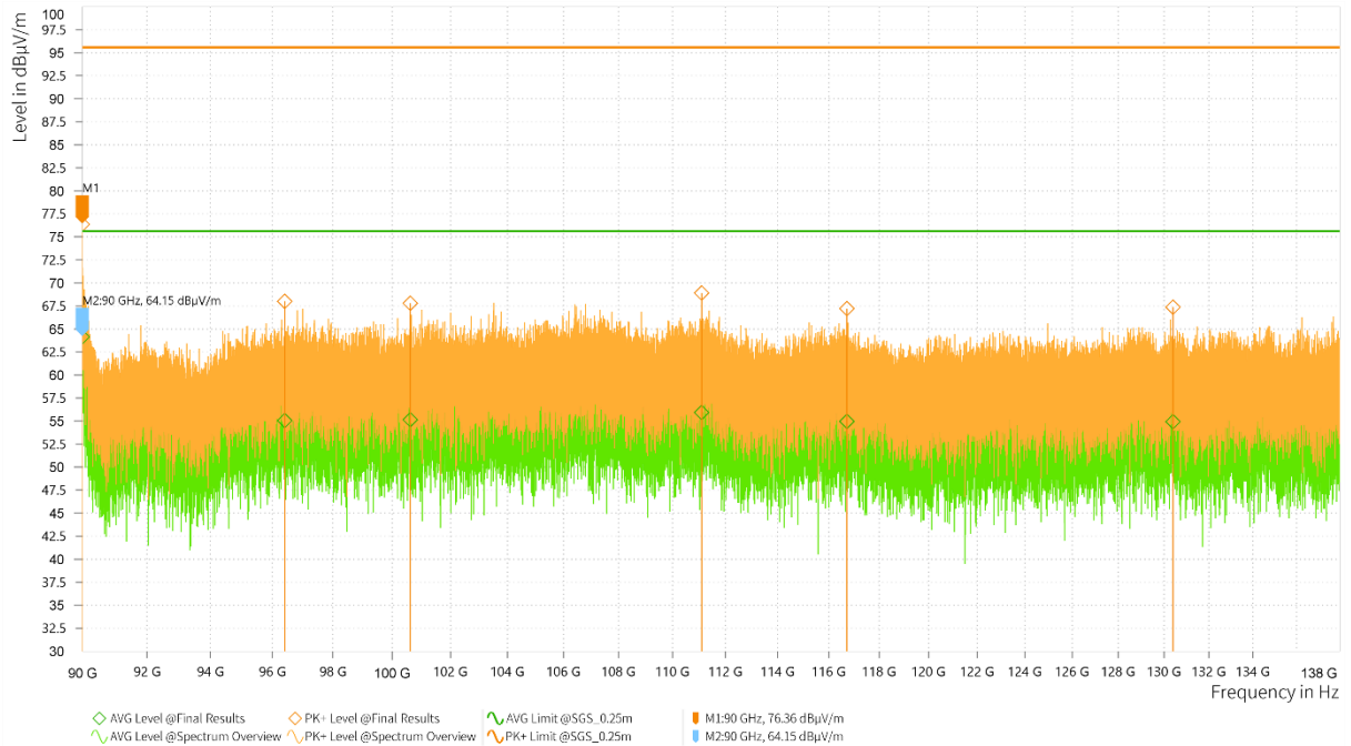
Antenna Polarity & Test Distance: Horizontal at 0.25 m
