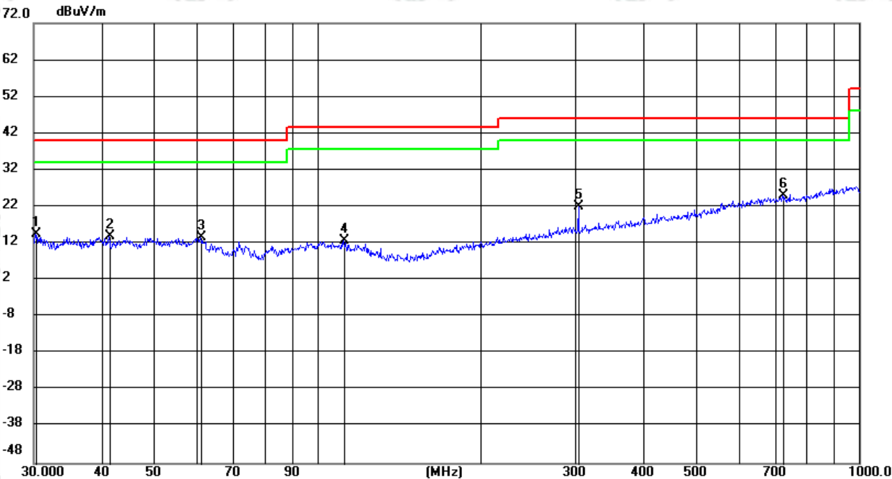
Test Graph Polarization: Horizontal
