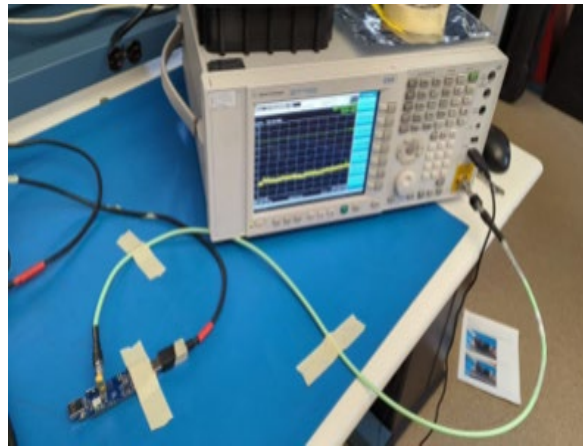
Conducted Measurements
