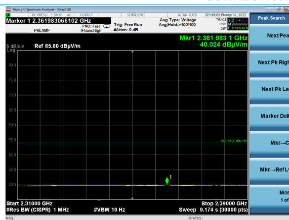
2310-2390 MHz, Average Horizontal EUT, BLE Ch. 1, Module 1
