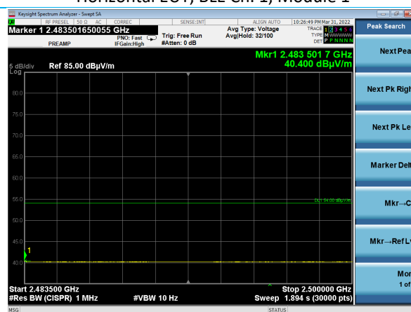
2483.5-2500 MHz, Average Horizontal EUT, BLE Ch. 39, Module 1
