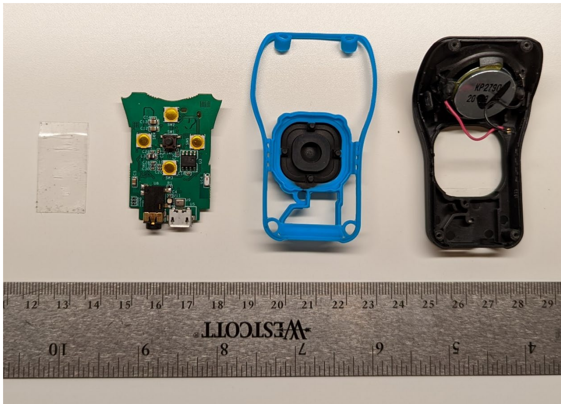
Circuit board removed from front housing
