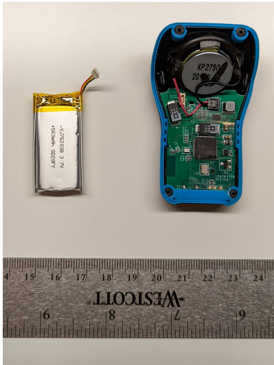
Battery removed
