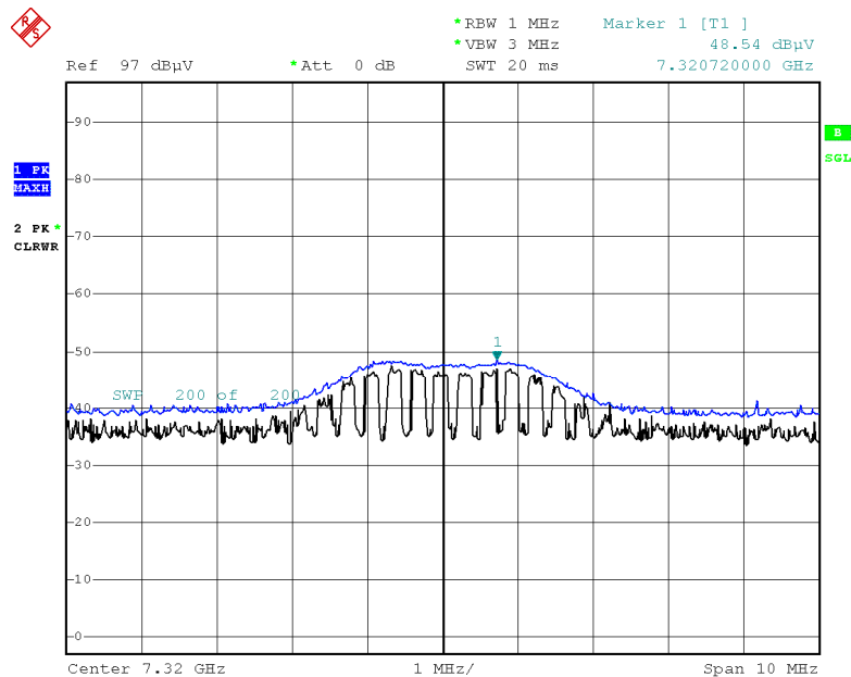
Radiated Spurious Emissions plot – Peak Measured Level (Ch.19 3rd Harmonic)
