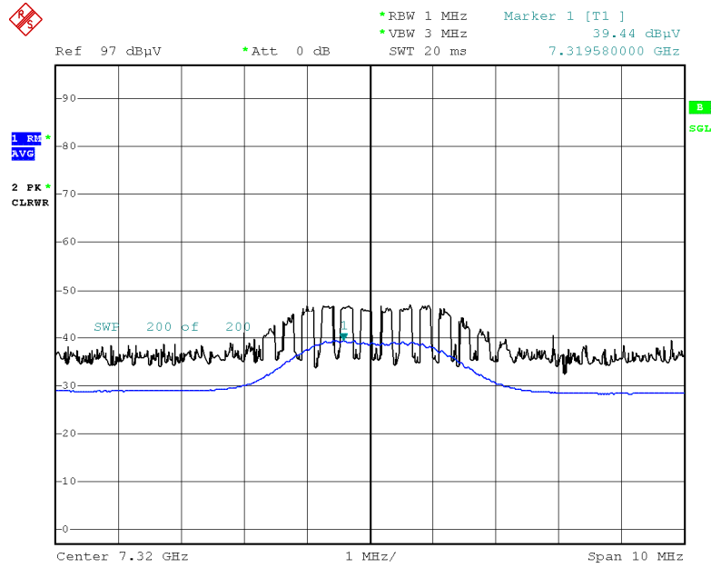
Radiated Spurious Emissions plot – Average Measured Level (Ch.19 3rd Harmonic)
