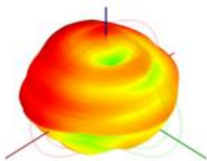
2441.0MHz H+V, Eff: 60.8%
