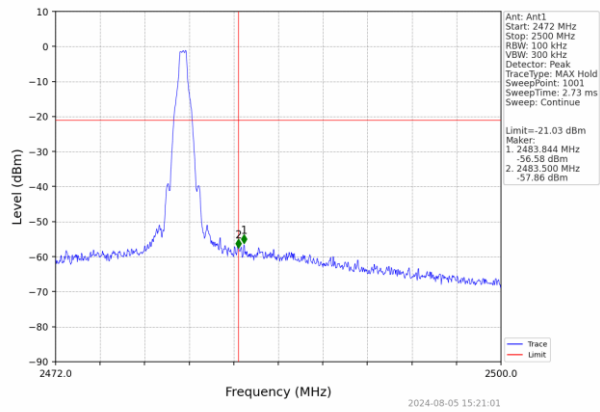
No-hopping mode
