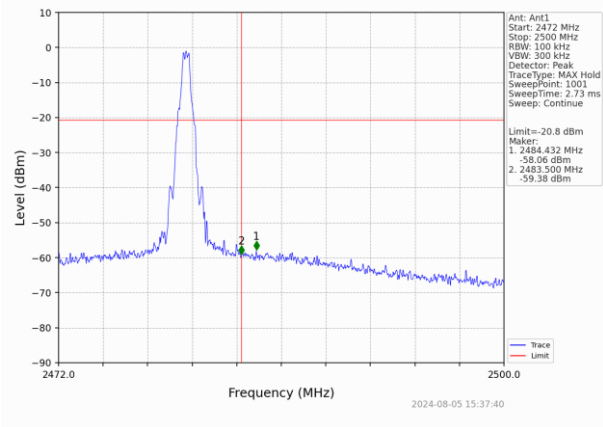
No-hopping mode
