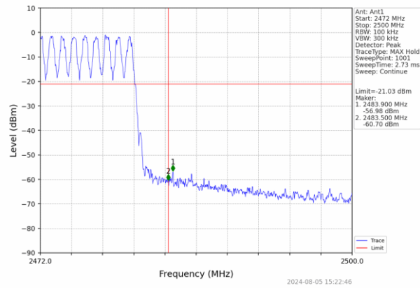
Hopping mode
