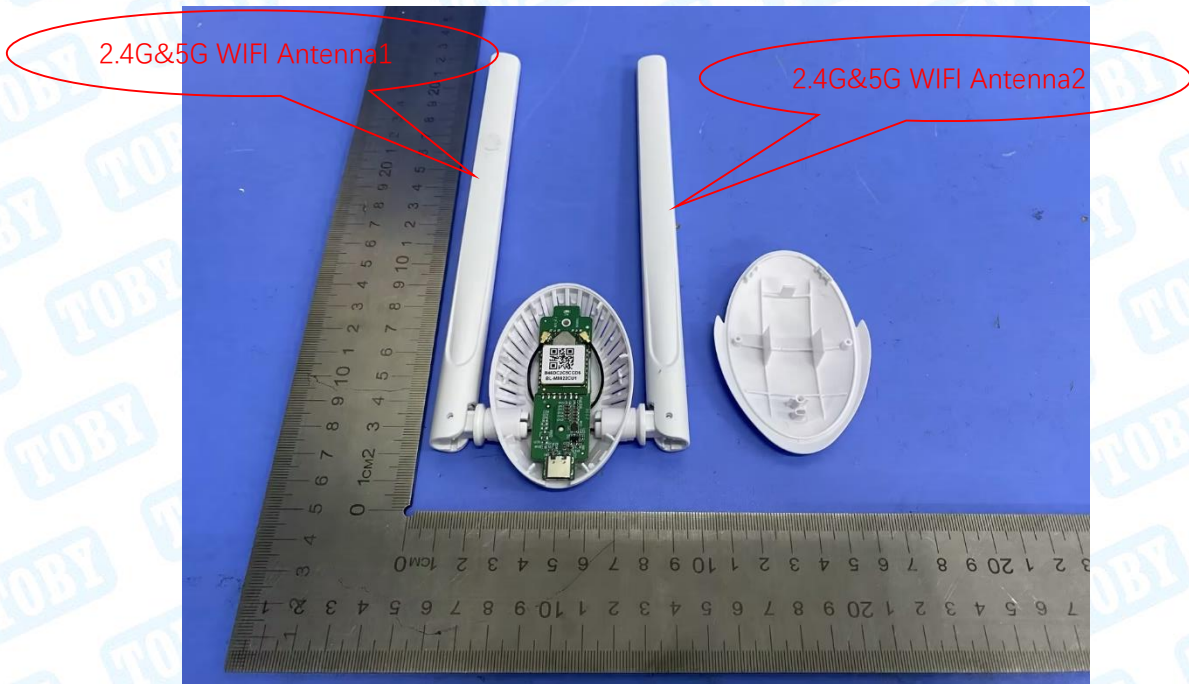
Photo 9 Appearance of PCB
