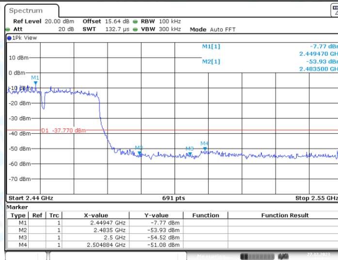
11N40MIMO_Ant1_High_2452
