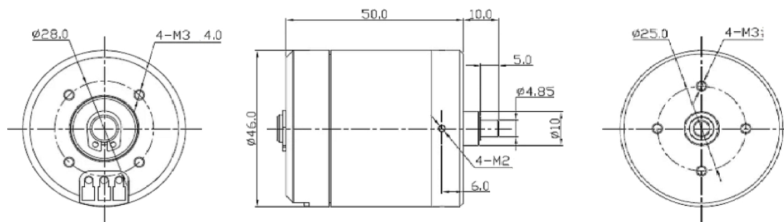
Motor Outline Drawing
